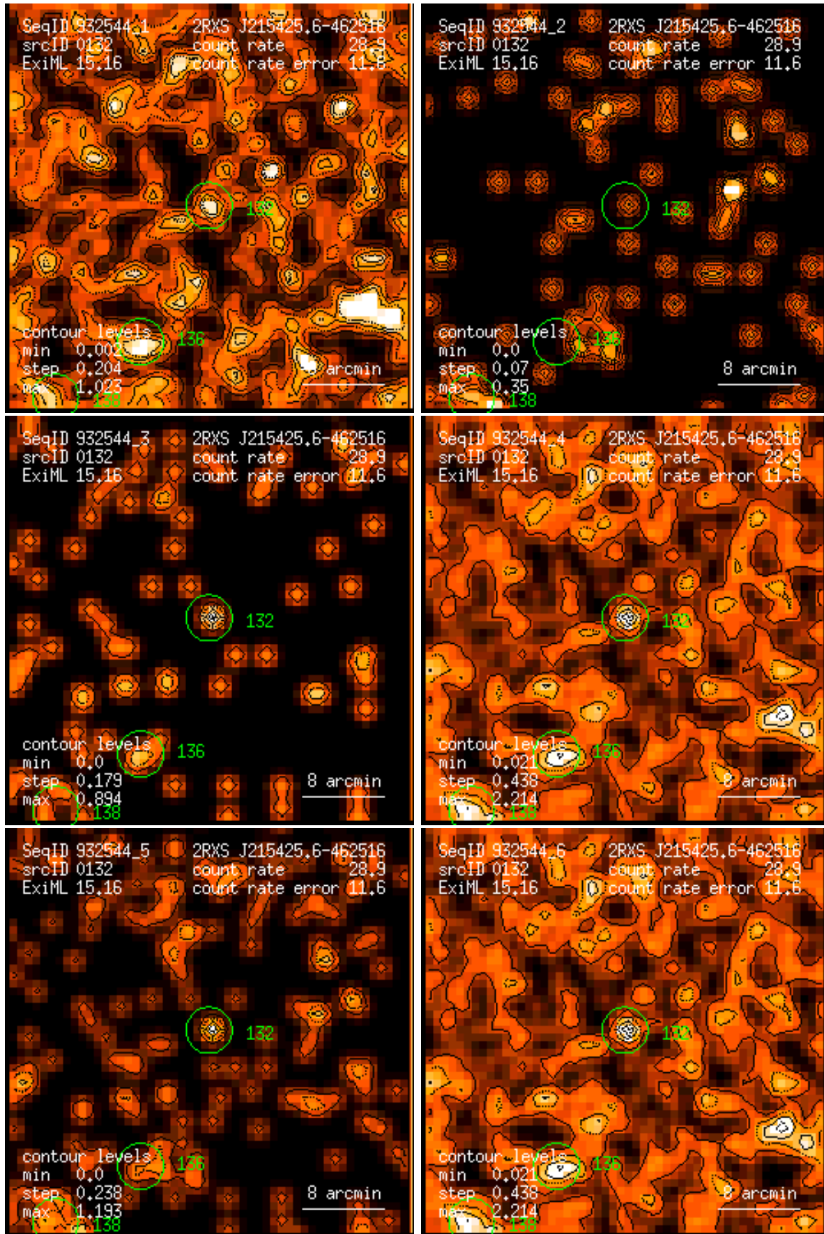
Figure 132: RASS 932544: detection 0132: band rate images, Gaussian filter: (1) PSPC channels 11 – 41, (2) 52 – 90, (3) 91 – 201, (4) 11 – 235, (5) 52 – 201, (6) 11 – 201. Broad band rates in counts/ks. Band rate contour levels in counts/ks/arcmin 2 .
