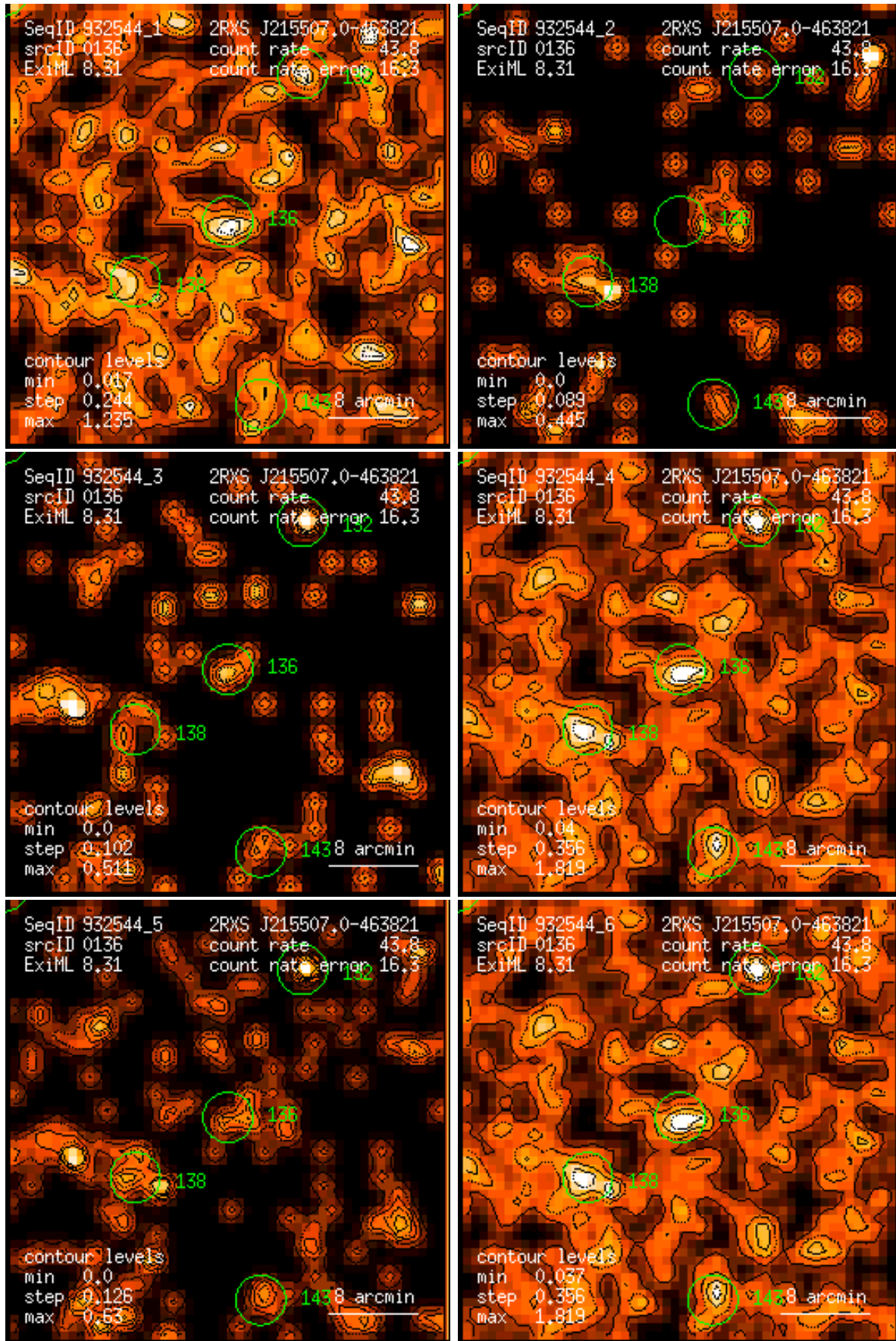
Figure 136: RASS 932544: detection 0136: band rate images, Gaussian filter: (1) PSPC channels 11 – 41, (2) 52 – 90, (3) 91 – 201, (4) 11 – 235, (5) 52 – 201, (6) 11 – 201. Broad band rates in counts/ks. Band rate contour levels in counts/ks/arcmin 2 .
