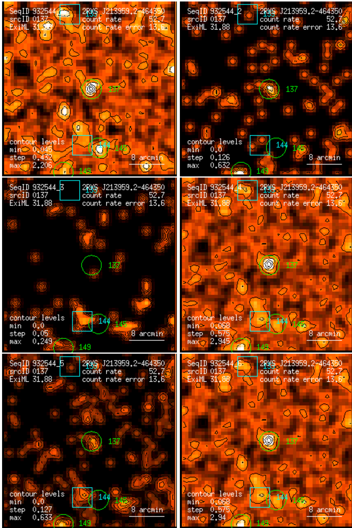
Figure 137: RASS 932544: detection 0137: band rate images, Gaussian filter: (1) PSPC channels 11 – 41, (2) 52 – 90, (3) 91 – 201, (4) 11 – 235, (5) 52 – 201, (6) 11 – 201. Broad band rates in counts/ks. Band rate contour levels in counts/ks/arcmin 2 .
