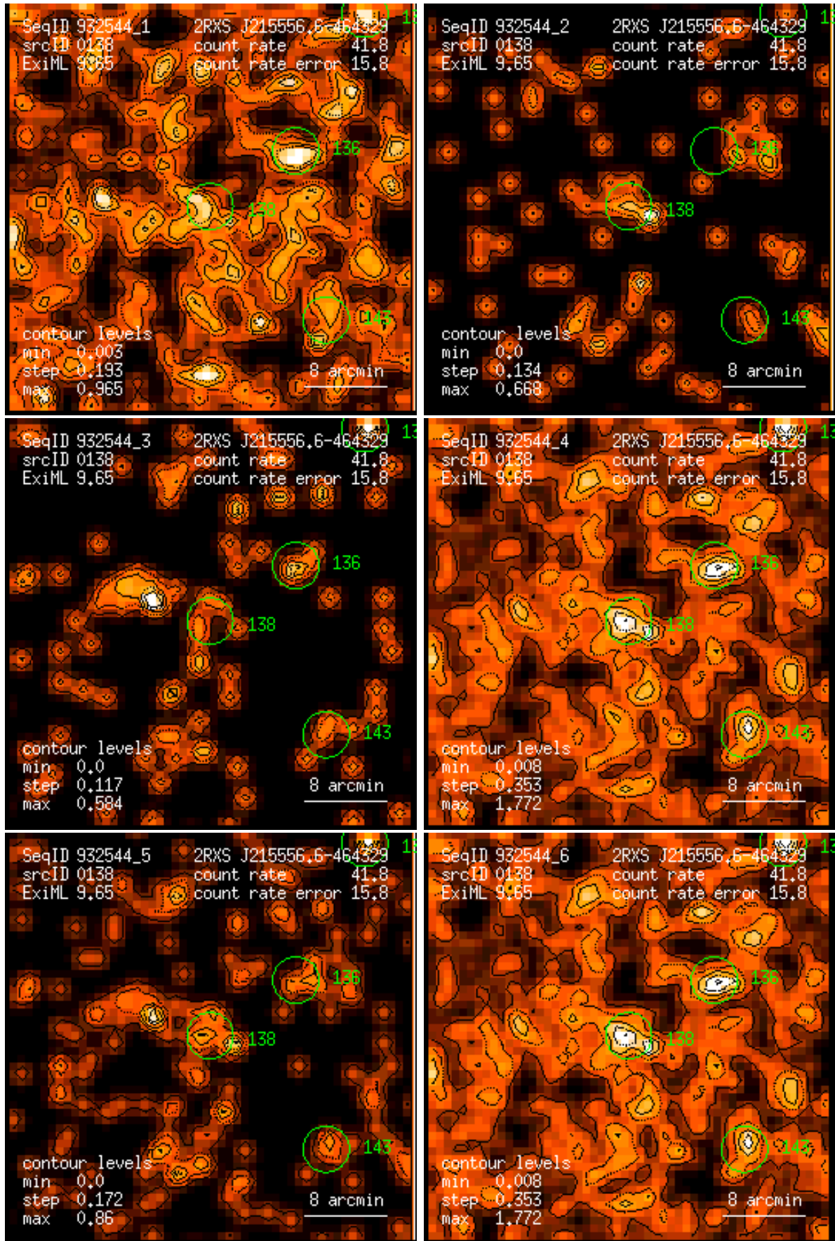
Figure 138: RASS 932544: detection 0138: band rate images, Gaussian filter: (1) PSPC channels 11 – 41, (2) 52 – 90, (3) 91 – 201, (4) 11 – 235, (5) 52 – 201, (6) 11 – 201. Broad band rates in counts/ks. Band rate contour levels in counts/ks/arcmin 2 .
