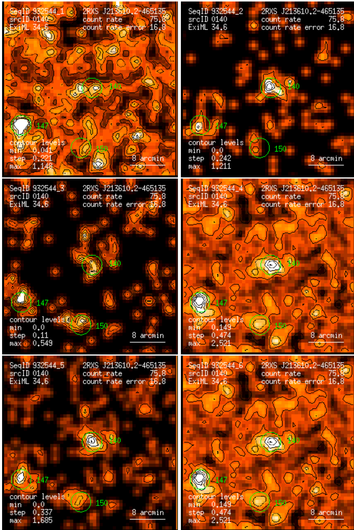
Figure 140: RASS 932544: detection 0140: band rate images, Gaussian filter: (1) PSPC channels 11 – 41, (2) 52 – 90, (3) 91 – 201, (4) 11 – 235, (5) 52 – 201, (6) 11 – 201. Broad band rates in counts/ks. Band rate contour levels in counts/ks/arcmin 2 .
