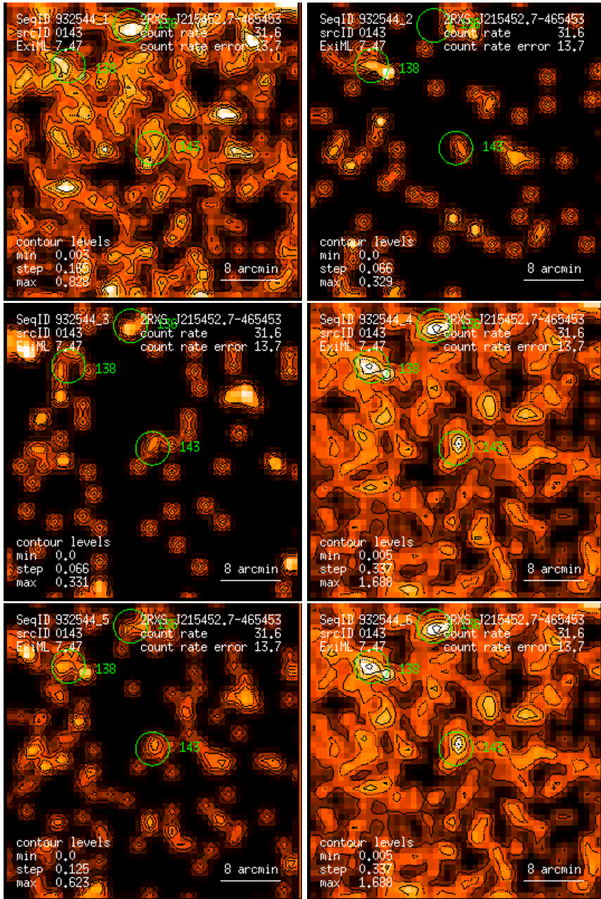
Figure 143: RASS 932544: detection 0143: band rate images, Gaussian filter: (1) PSPC channels 11 – 41, (2) 52 – 90, (3) 91 – 201, (4) 11 – 235, (5) 52 – 201, (6) 11 – 201. Broad band rates in counts/ks. Band rate contour levels in counts/ks/arcmin 2 .
