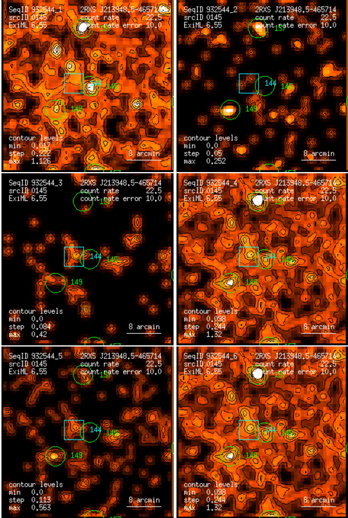
Figure 145: RASS 932544: detection 0145: band rate images, Gaussian filter: (1) PSPC channels 11 – 41, (2) 52 – 90, (3) 91 – 201, (4) 11 – 235, (5) 52 – 201, (6) 11 – 201. Broad band rates in counts/ks. Band rate contour levels in counts/ks/arcmin 2 .
