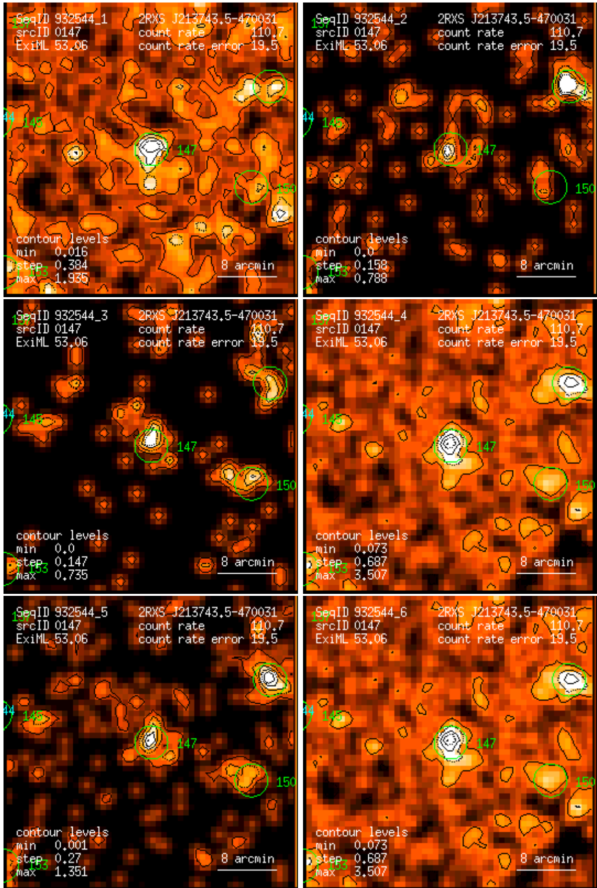
Figure 147: RASS 932544: detection 0147: band rate images, Gaussian filter: (1) PSPC channels 11 – 41, (2) 52 – 90, (3) 91 – 201, (4) 11 – 235, (5) 52 – 201, (6) 11 – 201. Broad band rates in counts/ks. Band rate contour levels in counts/ks/arcmin 2 .
