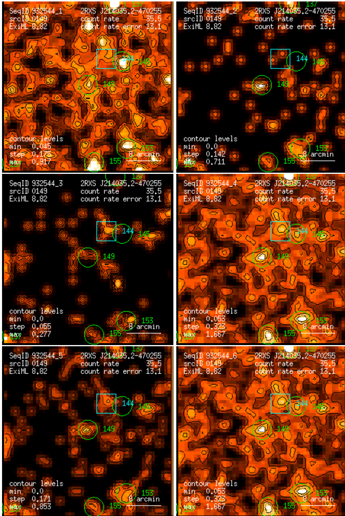
Figure 149: RASS 932544: detection 0149: band rate images, Gaussian filter: (1) PSPC channels 11 – 41, (2) 52 – 90, (3) 91 – 201, (4) 11 – 235, (5) 52 – 201, (6) 11 – 201. Broad band rates in counts/ks. Band rate contour levels in counts/ks/arcmin 2 .
