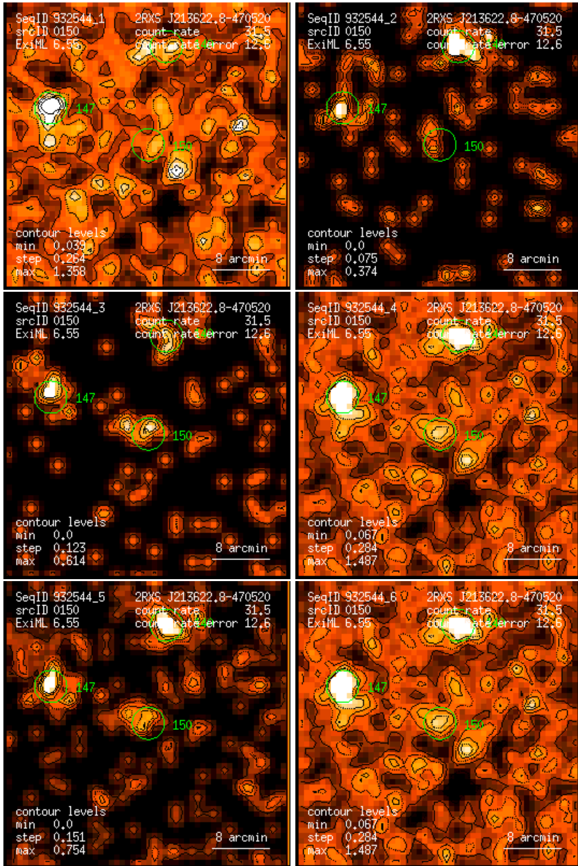
Figure 150: RASS 932544: detection 0150: band rate images, Gaussian filter: (1) PSPC channels 11 – 41, (2) 52 – 90, (3) 91 – 201, (4) 11 – 235, (5) 52 – 201, (6) 11 – 201. Broad band rates in counts/ks. Band rate contour levels in counts/ks/arcmin 2 .
