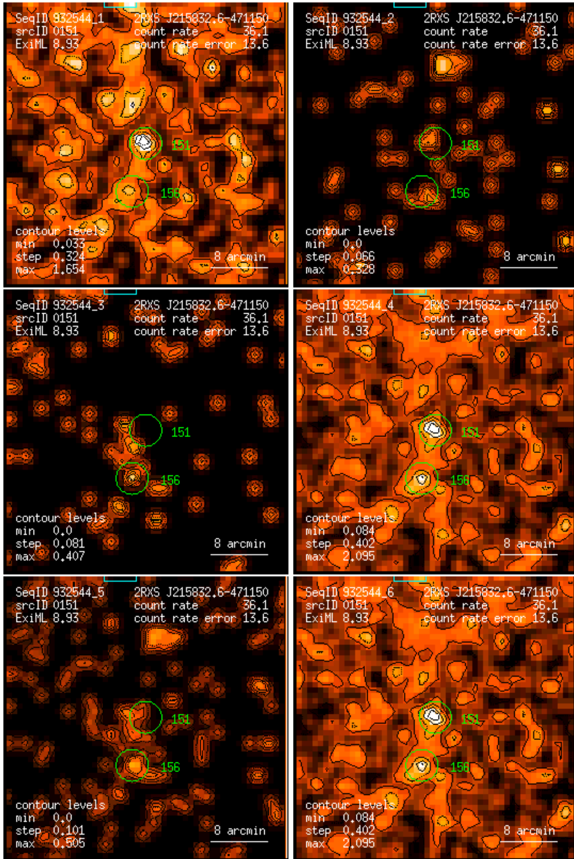
Figure 151: RASS 932544: detection 0151: band rate images, Gaussian filter: (1) PSPC channels 11 – 41, (2) 52 – 90, (3) 91 – 201, (4) 11 – 235, (5) 52 – 201, (6) 11 – 201. Broad band rates in counts/ks. Band rate contour levels in counts/ks/arcmin 2 .
