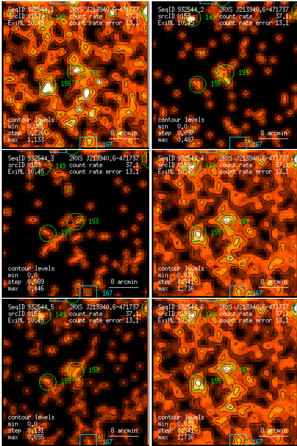
Figure 153: RASS 932544: detection 0153: band rate images, Gaussian filter: (1) PSPC channels 11 – 41, (2) 52 – 90, (3) 91 – 201, (4) 11 – 235, (5) 52 – 201, (6) 11 – 201. Broad band rates in counts/ks. Band rate contour levels in counts/ks/arcmin 2 .
