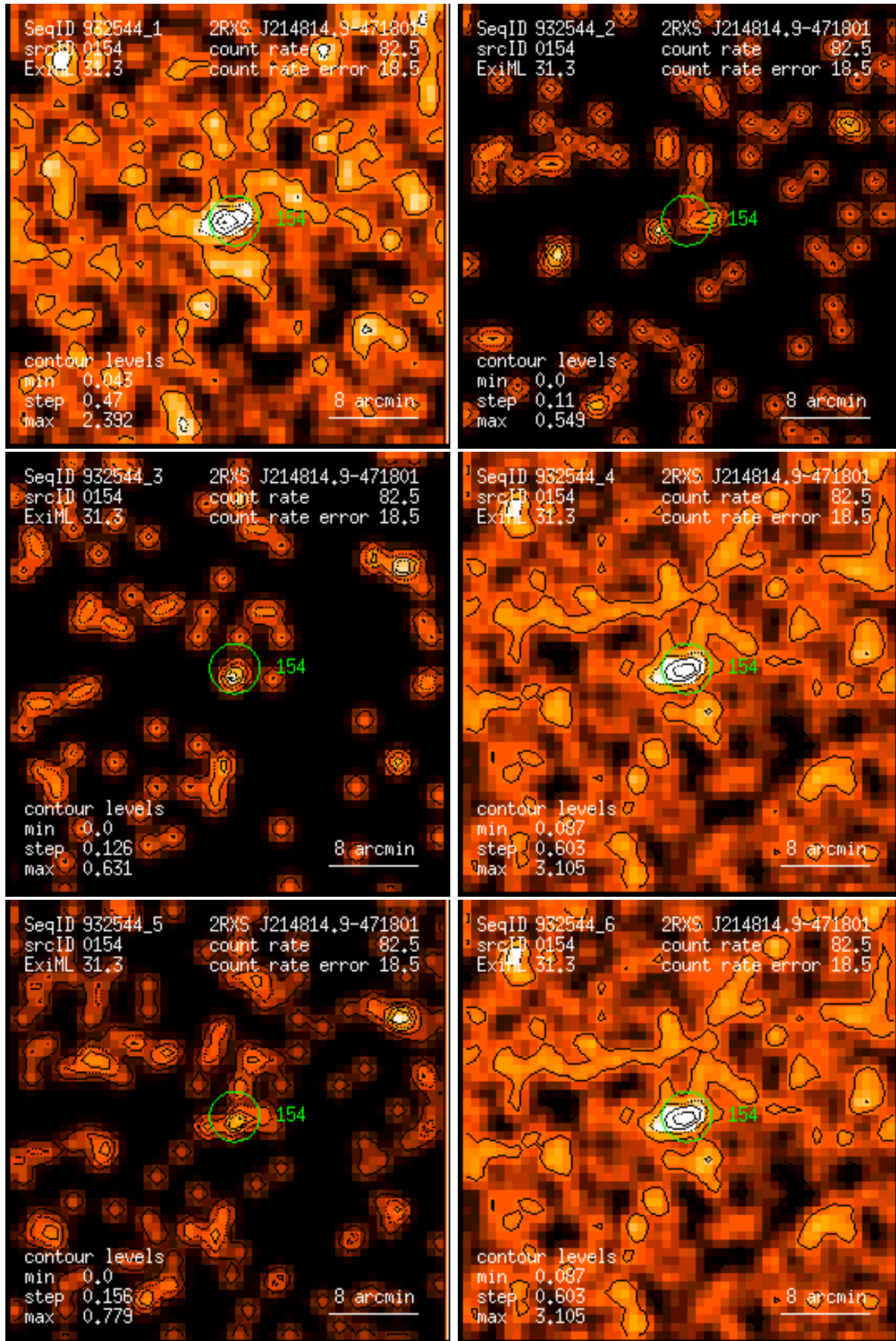
Figure 154: RASS 932544: detection 0154: band rate images, Gaussian filter: (1) PSPC channels 11 – 41, (2) 52 – 90, (3) 91 – 201, (4) 11 – 235, (5) 52 – 201, (6) 11 – 201. Broad band rates in counts/ks. Band rate contour levels in counts/ks/arcmin 2 .
