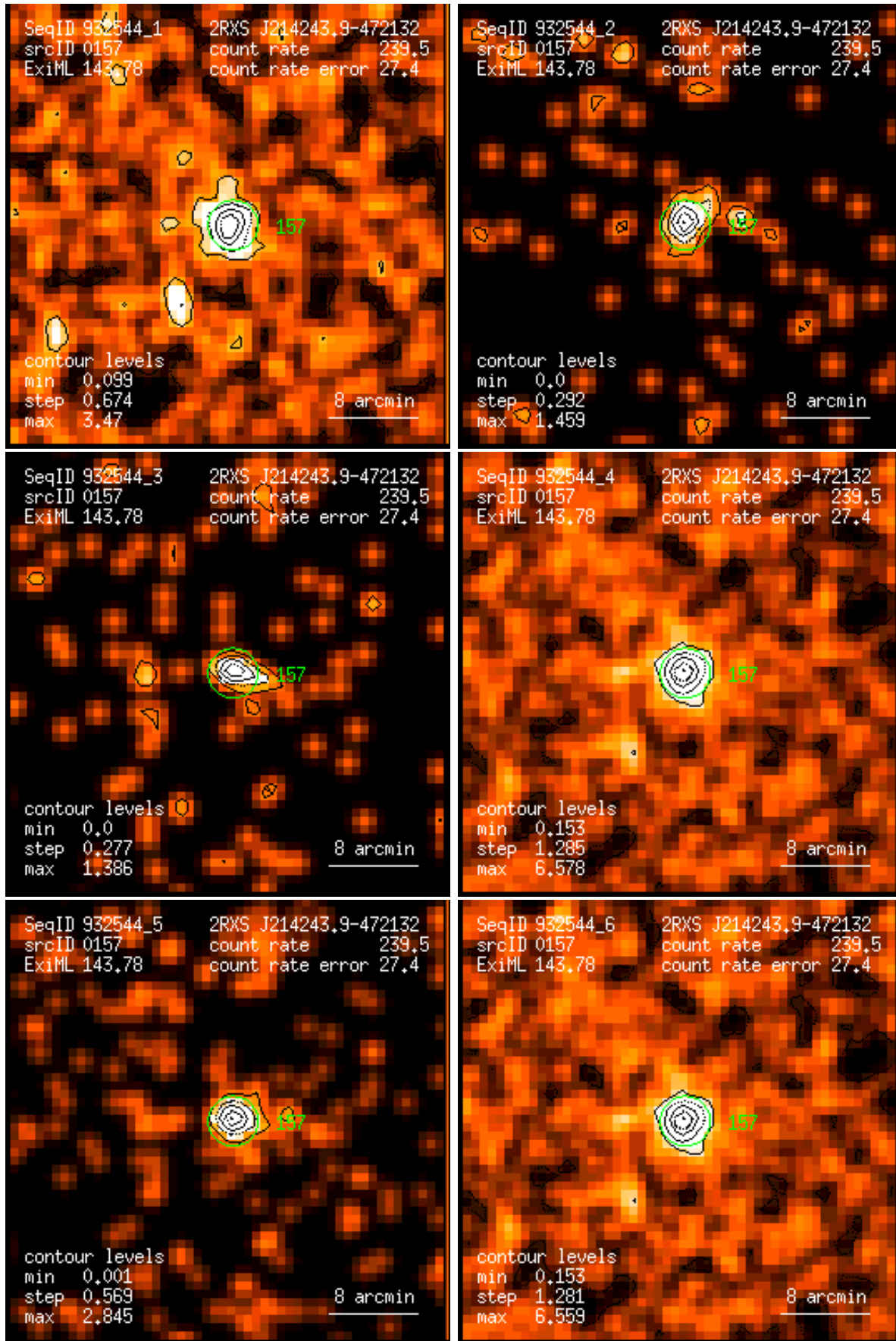
Figure 157: RASS 932544: detection 0157: band rate images, Gaussian filter: (1) PSPC channels 11 – 41, (2) 52 – 90, (3) 91 – 201, (4) 11 – 235, (5) 52 – 201, (6) 11 – 201. Broad band rates in counts/ks. Band rate contour levels in counts/ks/arcmin 2 .
