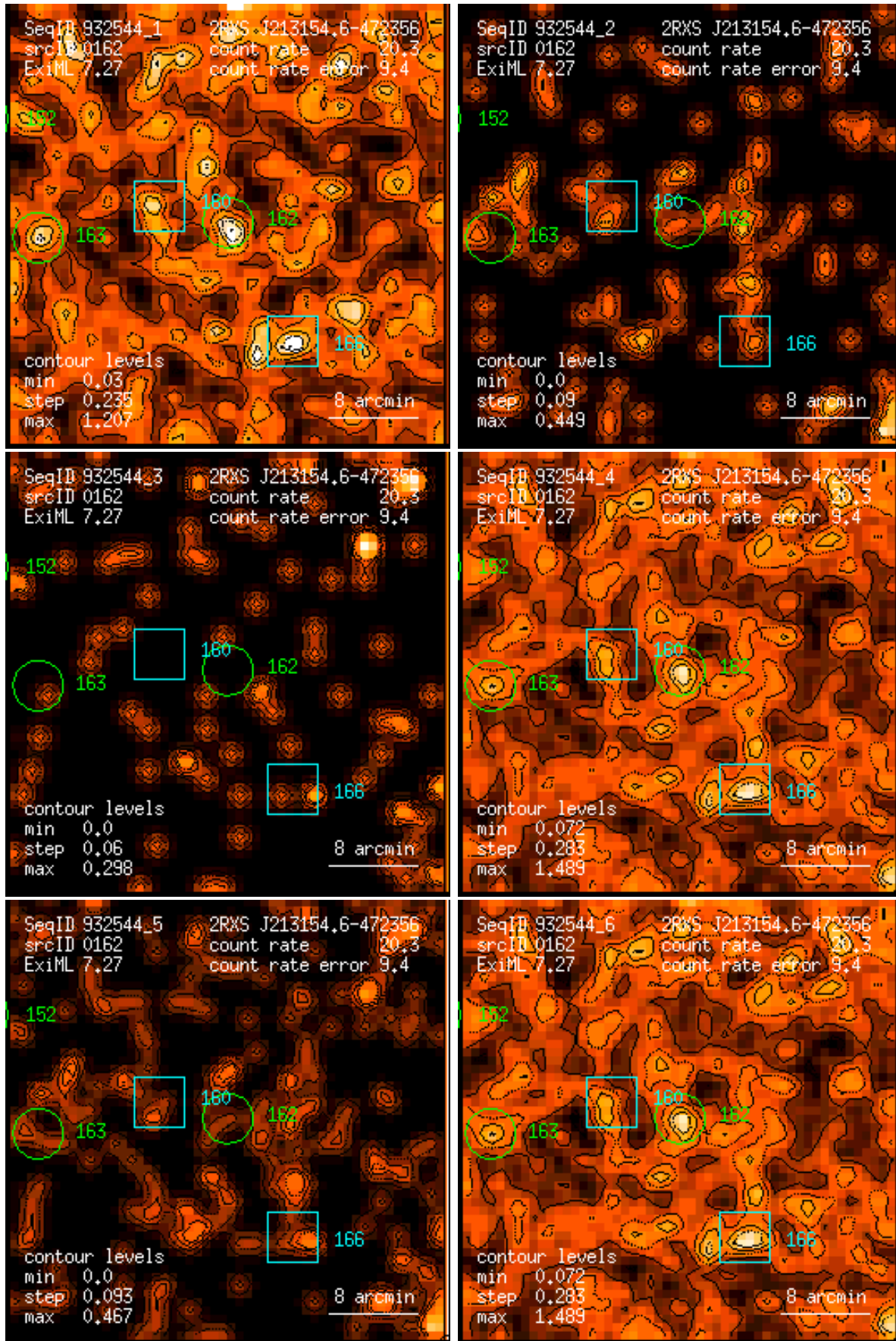
Figure 162: RASS 932544: detection 0162: band rate images, Gaussian filter: (1) PSPC channels 11 – 41, (2) 52 – 90, (3) 91 – 201, (4) 11 – 235, (5) 52 – 201, (6) 11 – 201. Broad band rates in counts/ks. Band rate contour levels in counts/ks/arcmin 2 .
