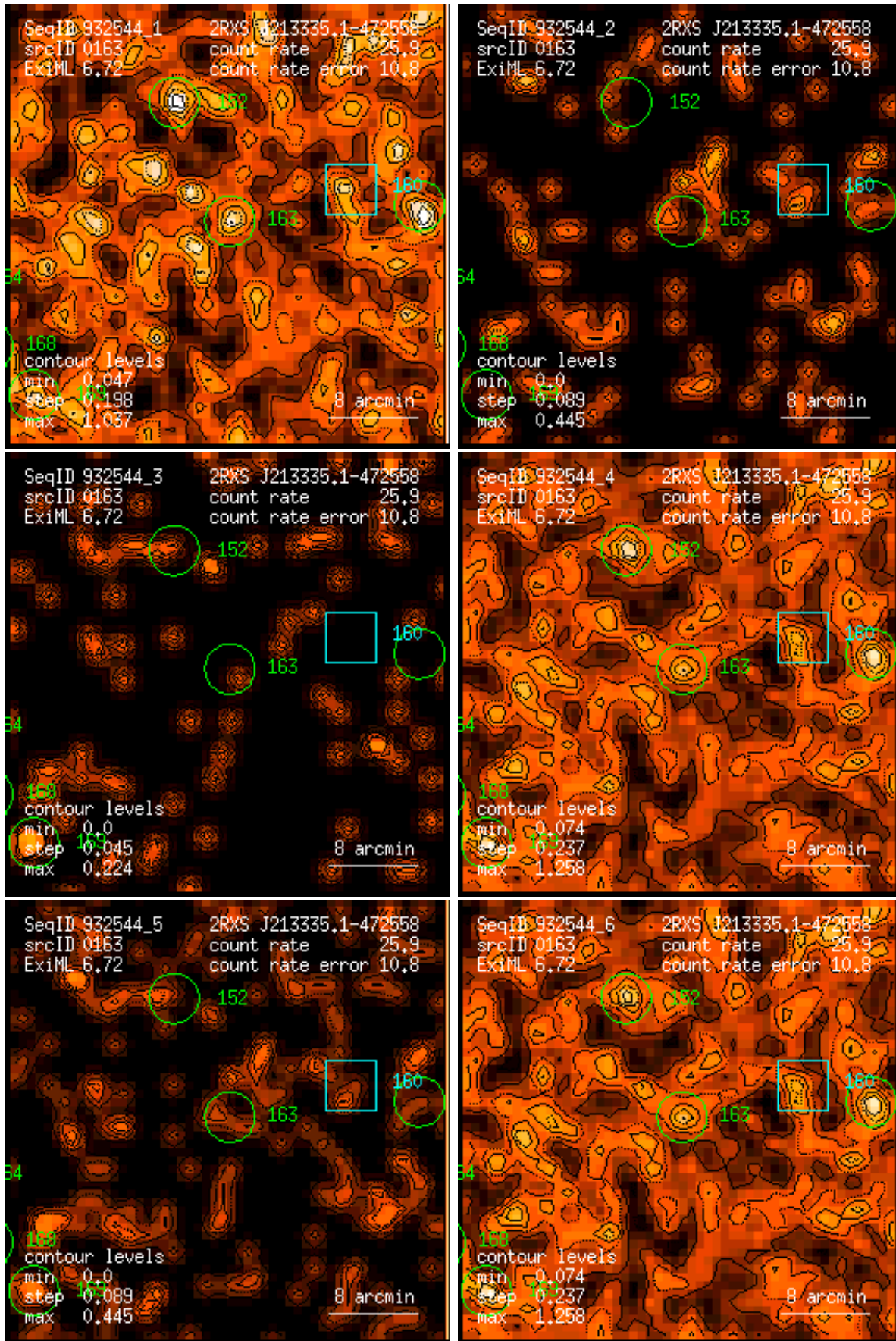
Figure 163: RASS 932544: detection 0163: band rate images, Gaussian filter: (1) PSPC channels 11 – 41, (2) 52 – 90, (3) 91 – 201, (4) 11 – 235, (5) 52 – 201, (6) 11 – 201. Broad band rates in counts/ks. Band rate contour levels in counts/ks/arcmin 2 .
