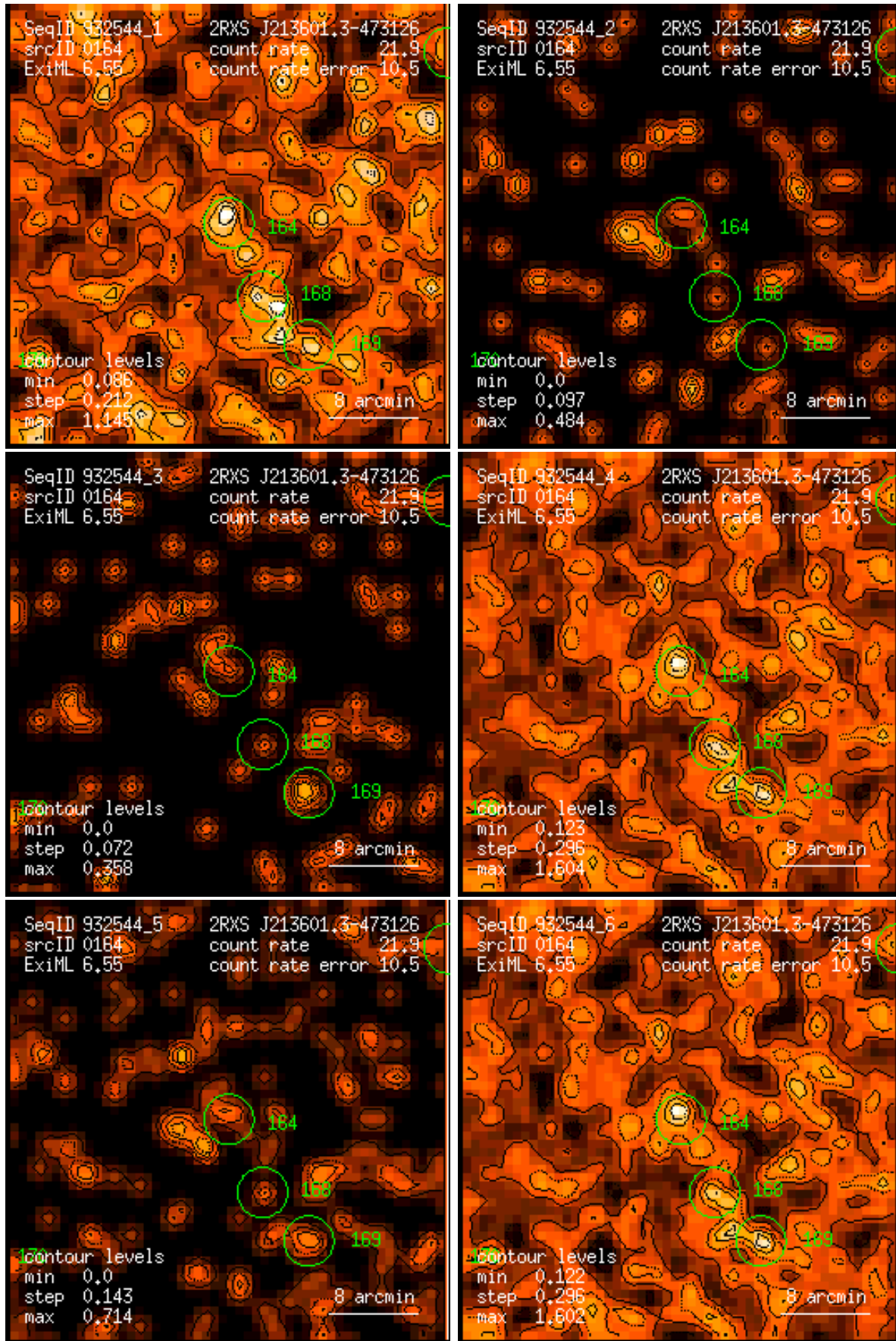
Figure 164: RASS 932544: detection 0164: band rate images, Gaussian filter: (1) PSPC channels 11 – 41, (2) 52 – 90, (3) 91 – 201, (4) 11 – 235, (5) 52 – 201, (6) 11 – 201. Broad band rates in counts/ks. Band rate contour levels in counts/ks/arcmin 2 .
