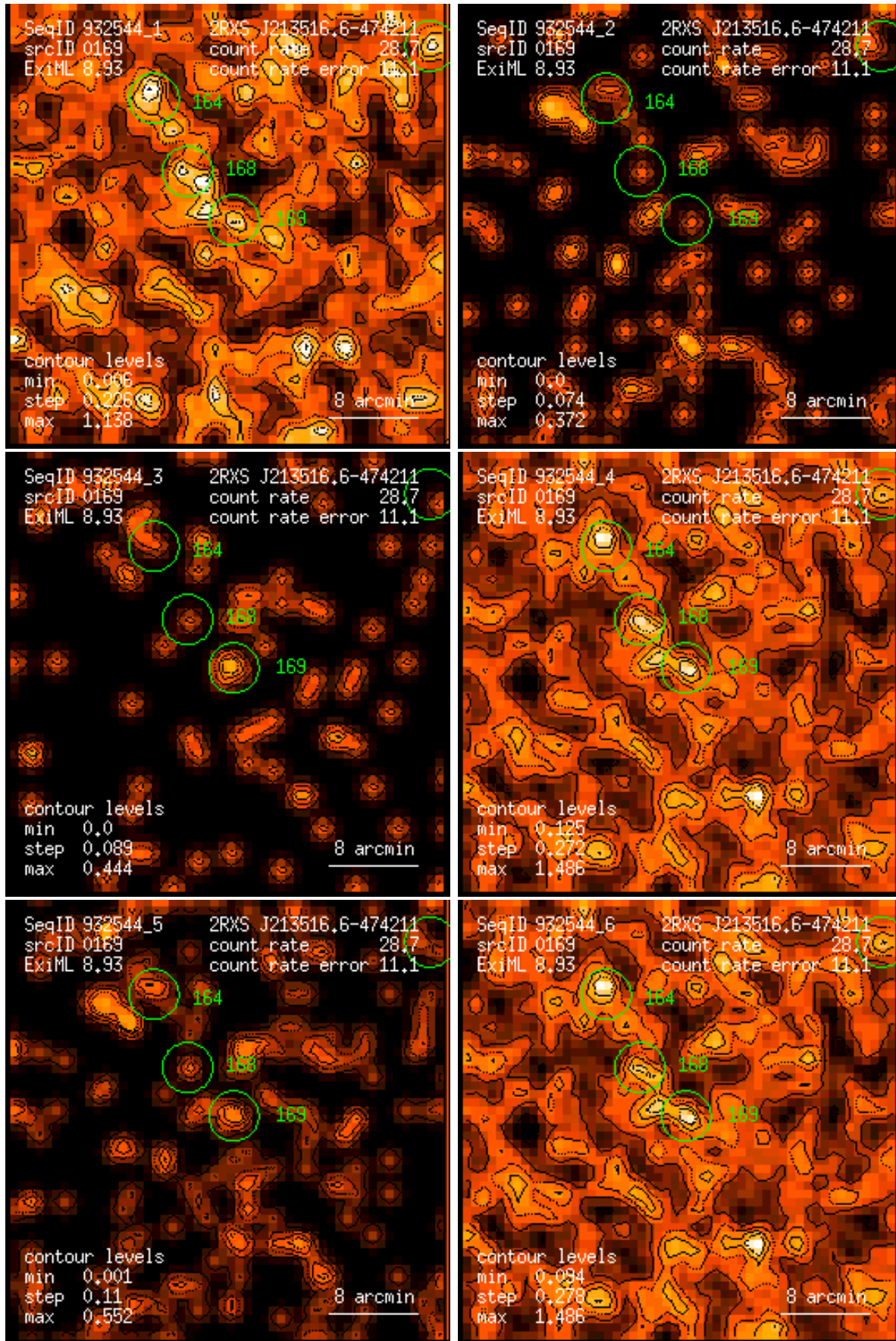
Figure 169: RASS 932544: detection 0169: band rate images, Gaussian filter: (1) PSPC channels 11 – 41, (2) 52 – 90, (3) 91 – 201, (4) 11 – 235, (5) 52 – 201, (6) 11 – 201. Broad band rates in counts/ks. Band rate contour levels in counts/ks/arcmin 2 .
