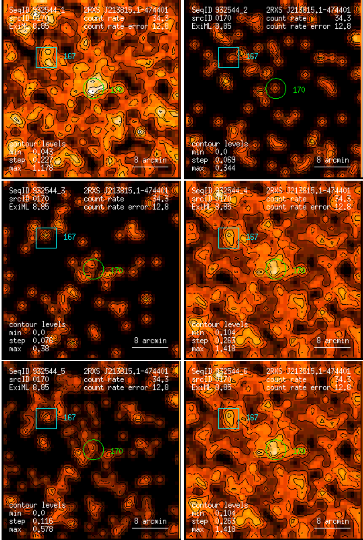
Figure 170: RASS 932544: detection 0170: band rate images, Gaussian filter: (1) PSPC channels 11 – 41, (2) 52 – 90, (3) 91 – 201, (4) 11 – 235, (5) 52 – 201, (6) 11 – 201. Broad band rates in counts/ks. Band rate contour levels in counts/ks/arcmin 2 .
