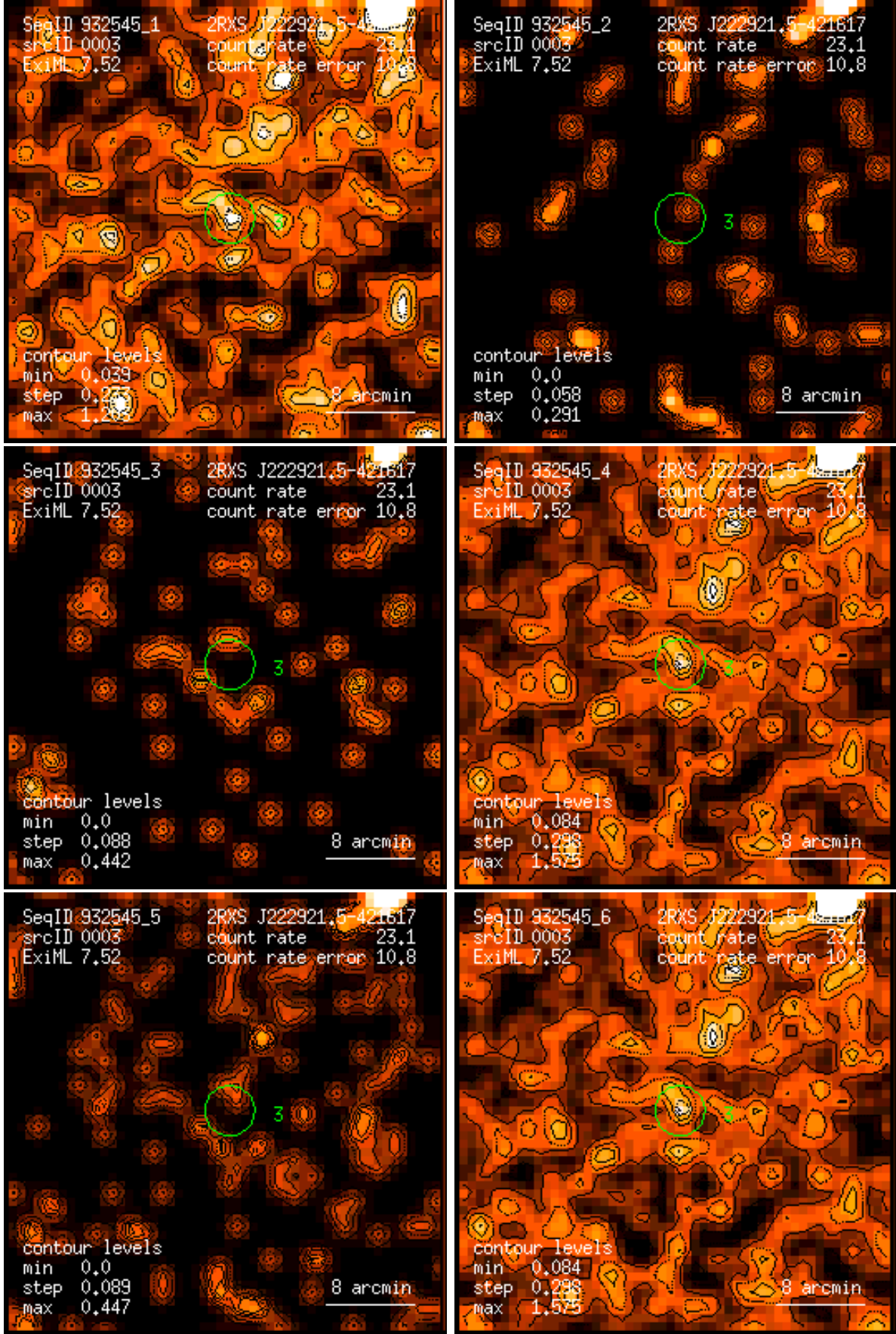
Figure 3: RASS 932545: detection 0003: band rate images, Gaussian filter: (1) PSPC channels 11 – 41, (2) 52 – 90, (3) 91 – 201, (4) 11 – 235, (5) 52 – 201, (6) 11 – 201. Broad band rates in counts/ks. Band rate contour levels in counts/ks/arcmin 2 .
