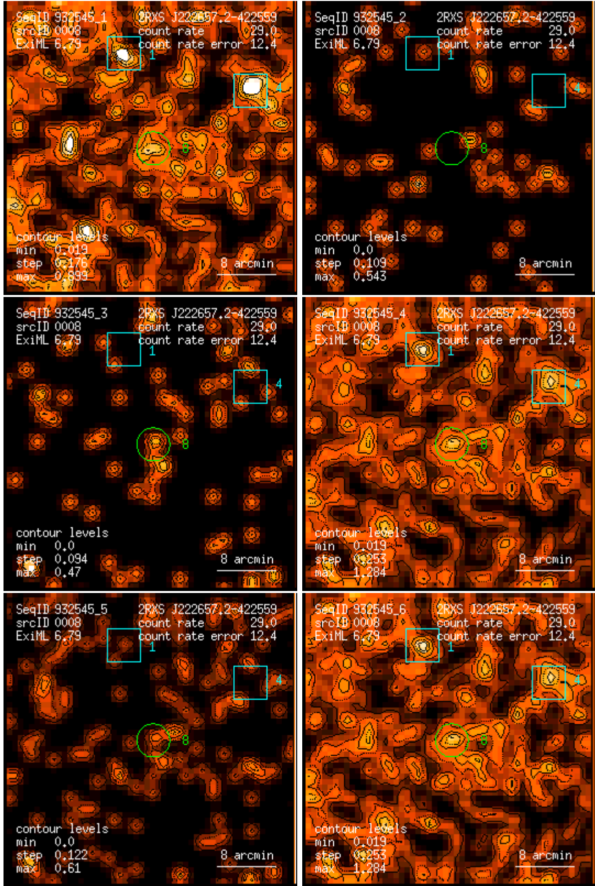
Figure 8: RASS 932545: detection 0008: band rate images, Gaussian filter: (1) PSPC channels 11 – 41, (2) 52 – 90, (3) 91 – 201, (4) 11 – 235, (5) 52 – 201, (6) 11 – 201. Broad band rates in counts/ks. Band rate contour levels in counts/ks/arcmin 2 .
