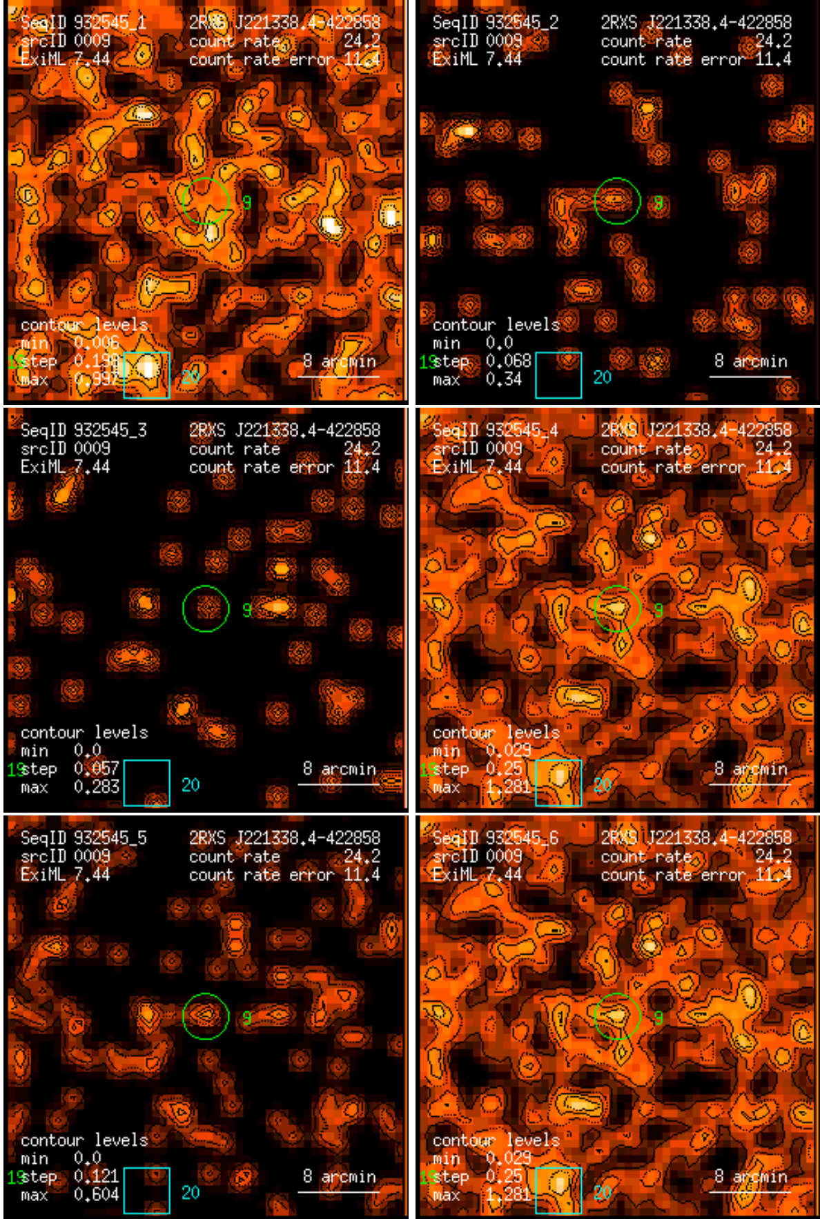
Figure 9: RASS 932545: detection 0009: band rate images, Gaussian filter: (1) PSPC channels 11 – 41, (2) 52 – 90, (3) 91 – 201, (4) 11 – 235, (5) 52 – 201, (6) 11 – 201. Broad band rates in counts/ks. Band rate contour levels in counts/ks/arcmin 2 .
