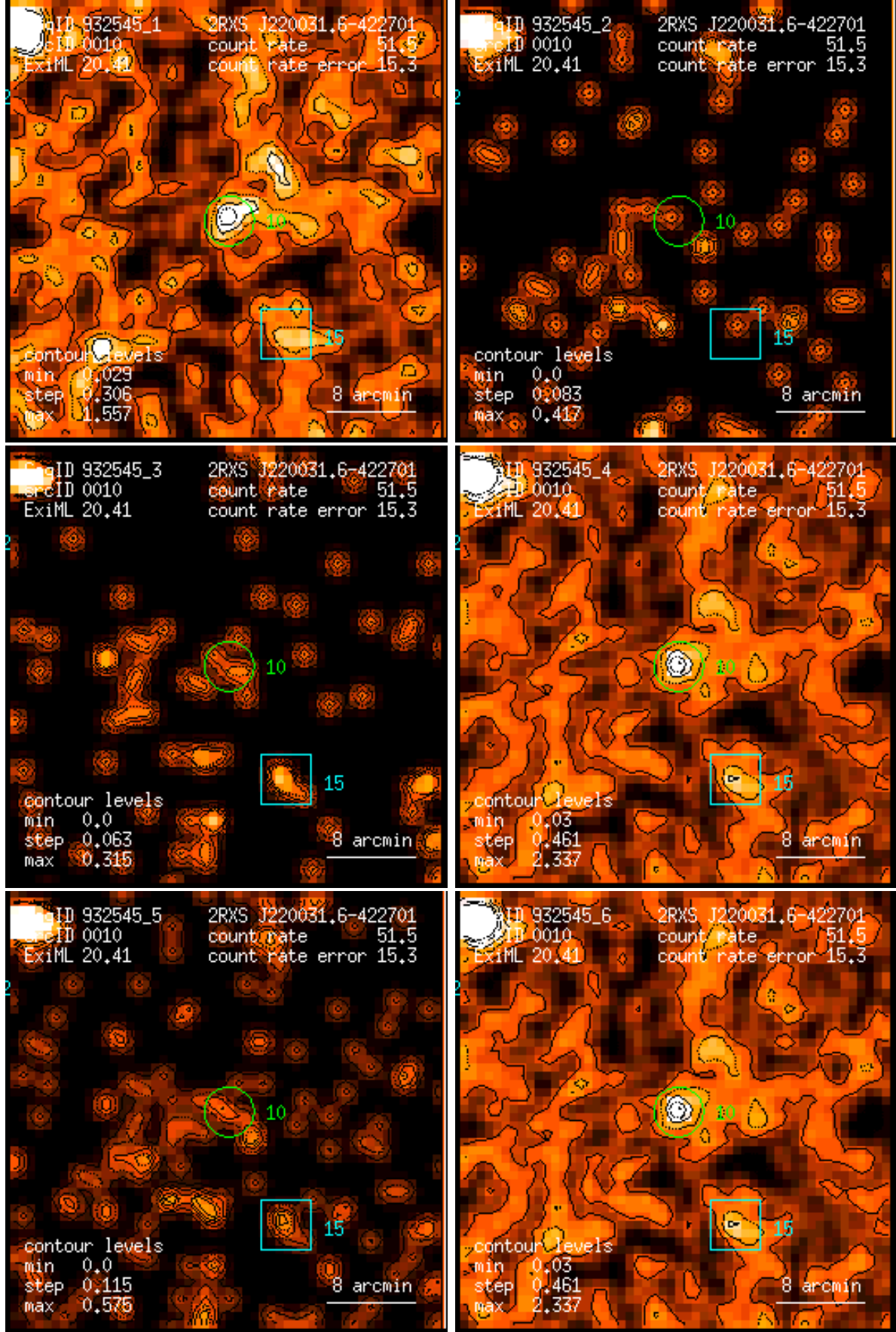
Figure 10: RASS 932545: detection 0010: band rate images, Gaussian filter: (1) PSPC channels 11 – 41, (2) 52 – 90, (3) 91 – 201, (4) 11 – 235, (5) 52 – 201, (6) 11 – 201. Broad band rates in counts/ks. Band rate contour levels in counts/ks/arcmin 2 .
