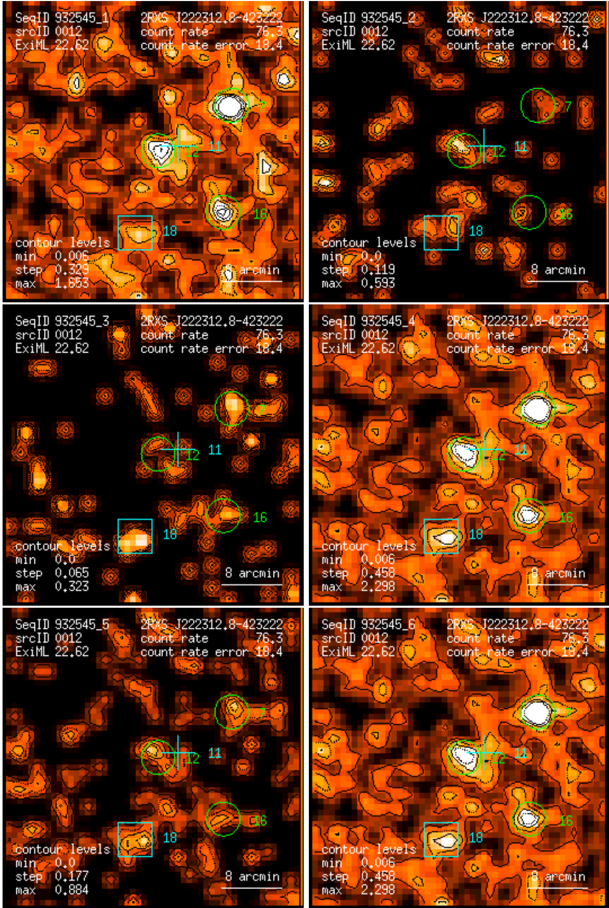
Figure 12: RASS 932545: detection 0012: band rate images, Gaussian filter: (1) PSPC channels 11 – 41, (2) 52 – 90, (3) 91 – 201, (4) 11 – 235, (5) 52 – 201, (6) 11 – 201. Broad band rates in counts/ks. Band rate contour levels in counts/ks/arcmin 2 .
