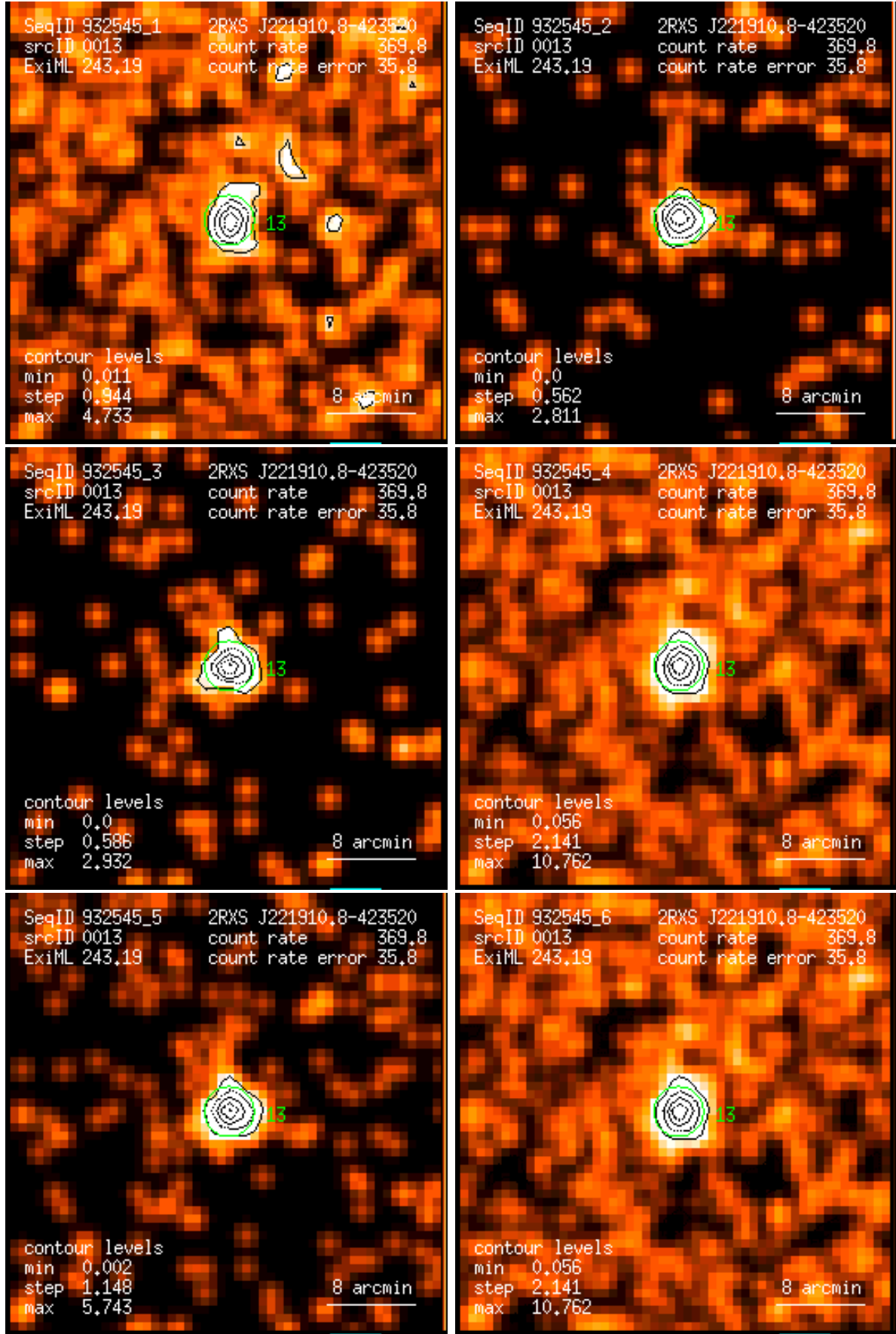
Figure 13: RASS 932545: detection 0013: band rate images, Gaussian filter: (1) PSPC channels 11 – 41, (2) 52 – 90, (3) 91 – 201, (4) 11 – 235, (5) 52 – 201, (6) 11 – 201. Broad band rates in counts/ks. Band rate contour levels in counts/ks/arcmin 2 .
