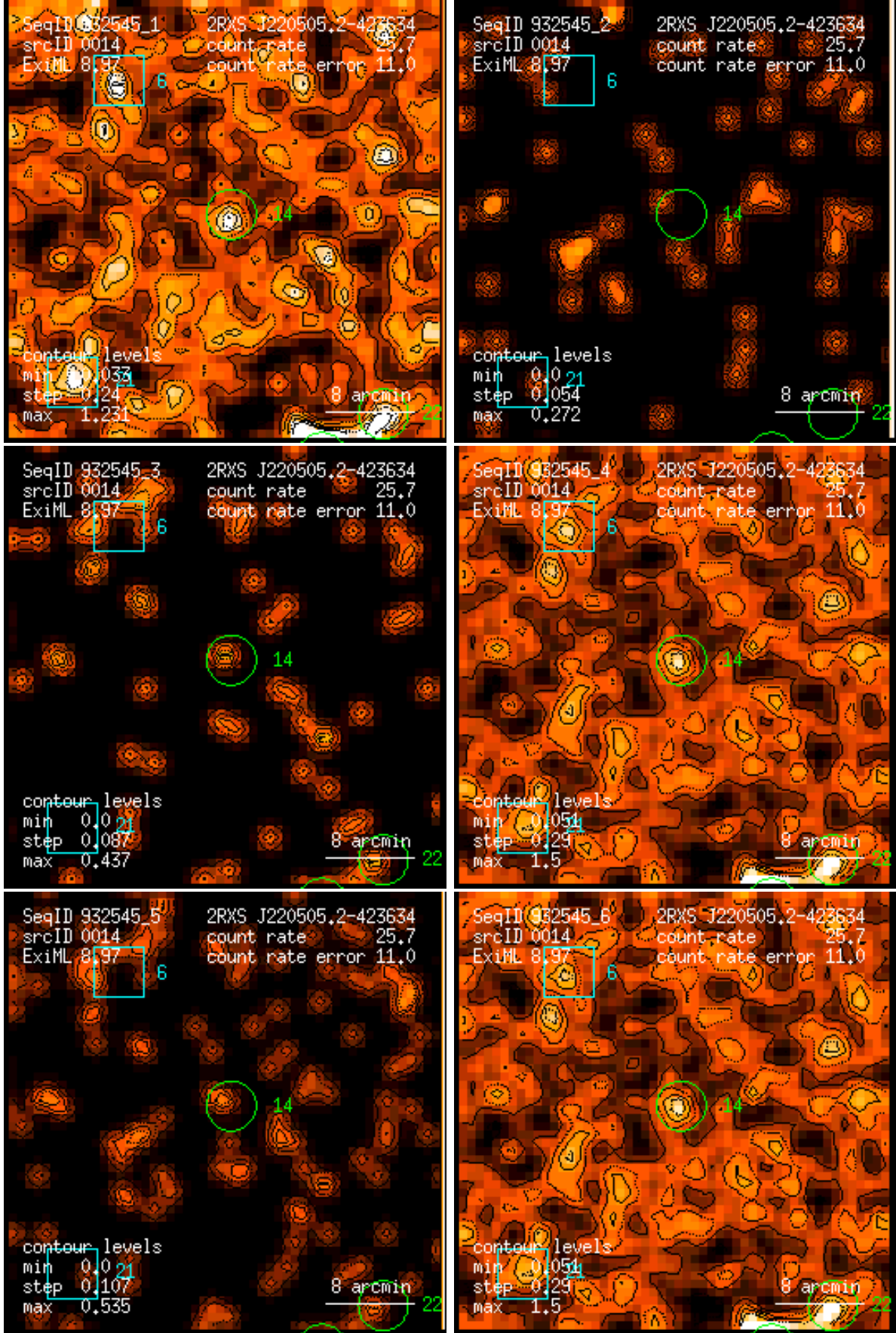
Figure 14: RASS 932545: detection 0014: band rate images, Gaussian filter: (1) PSPC channels 11 – 41, (2) 52 – 90, (3) 91 – 201, (4) 11 – 235, (5) 52 – 201, (6) 11 – 201. Broad band rates in counts/ks. Band rate contour levels in counts/ks/arcmin 2 .
