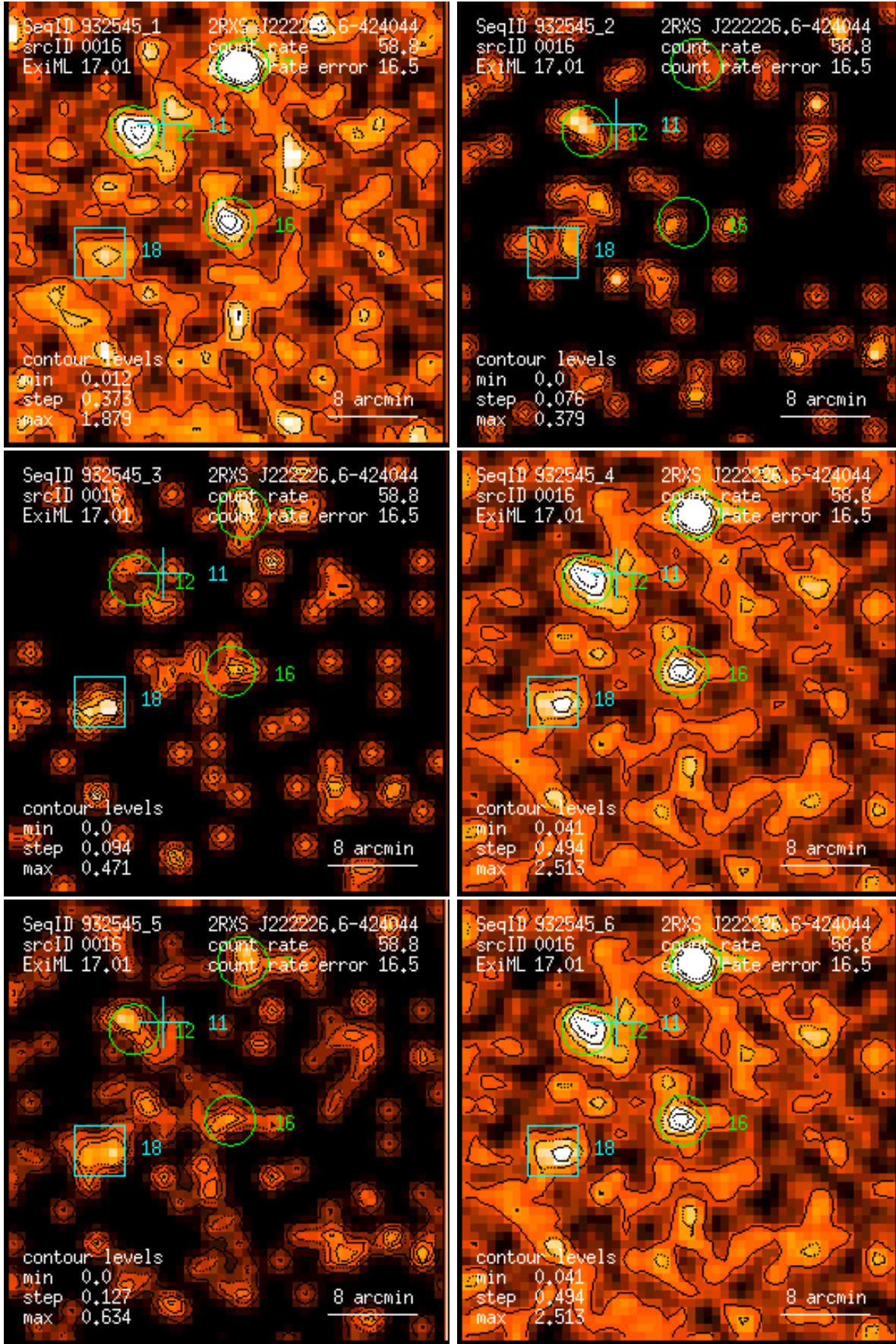
Figure 16: RASS 932545: detection 0016: band rate images, Gaussian filter: (1) PSPC channels 11 – 41, (2) 52 – 90, (3) 91 – 201, (4) 11 – 235, (5) 52 – 201, (6) 11 – 201. Broad band rates in counts/ks. Band rate contour levels in counts/ks/arcmin 2 .
