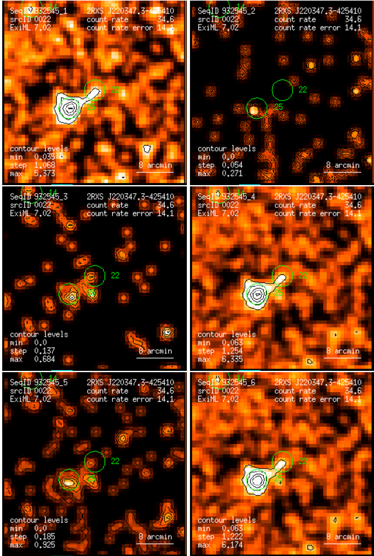
Figure 22: RASS 932545: detection 0022: band rate images, Gaussian filter: (1) PSPC channels 11 – 41, (2) 52 – 90, (3) 91 – 201, (4) 11 – 235, (5) 52 – 201, (6) 11 – 201. Broad band rates in counts/ks. Band rate contour levels in counts/ks/arcmin 2 .
