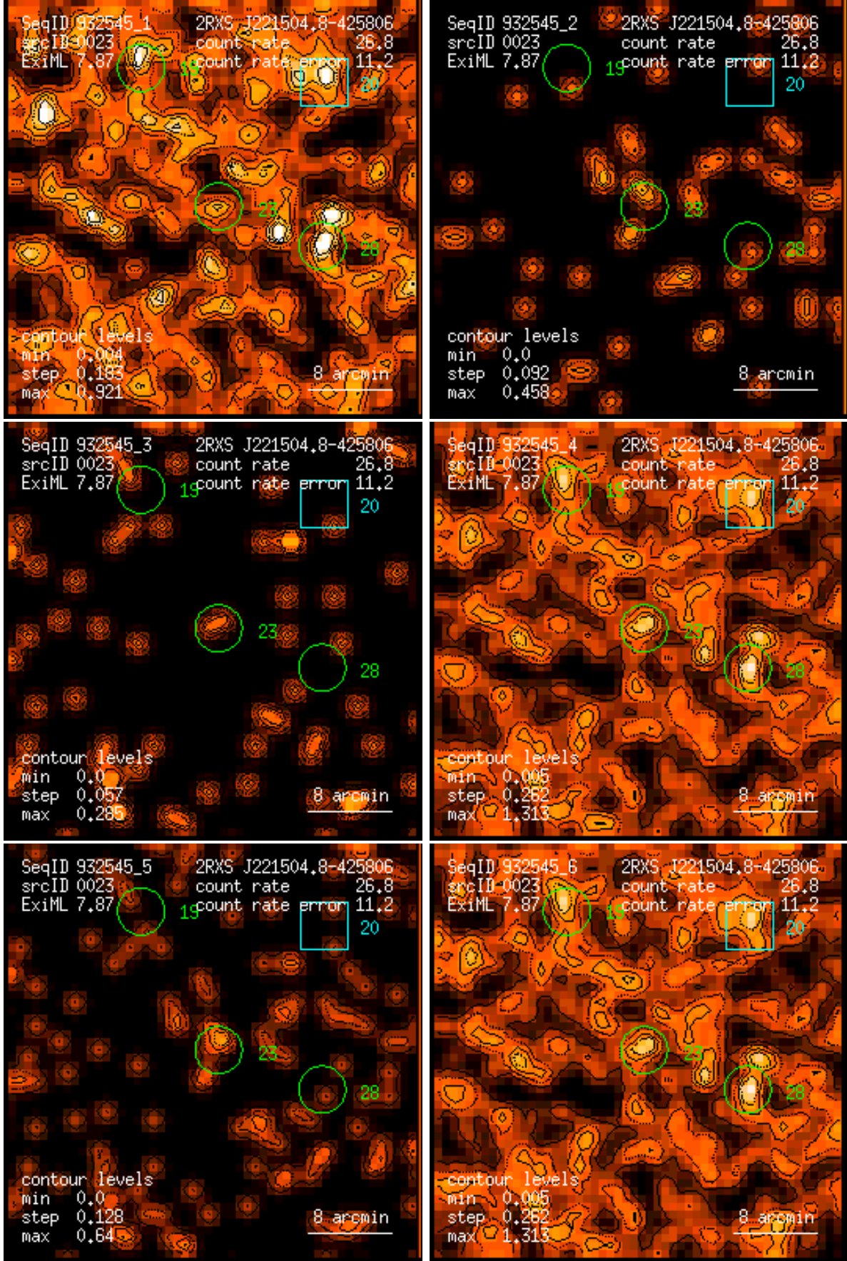
Figure 23: RASS 932545: detection 0023: band rate images, Gaussian filter: (1) PSPC channels 11 – 41, (2) 52 – 90, (3) 91 – 201, (4) 11 – 235, (5) 52 – 201, (6) 11 – 201. Broad band rates in counts/ks. Band rate contour levels in counts/ks/arcmin 2 .
