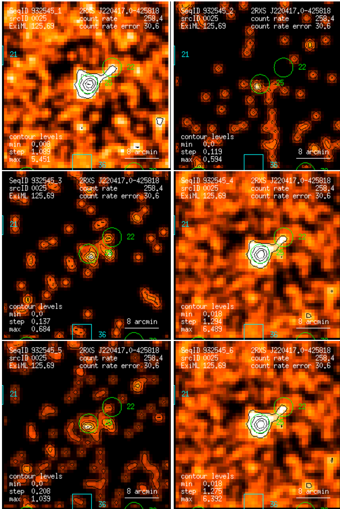
Figure 25: RASS 932545: detection 0025: band rate images, Gaussian filter: (1) PSPC channels 11 – 41, (2) 52 – 90, (3) 91 – 201, (4) 11 – 235, (5) 52 – 201, (6) 11 – 201. Broad band rates in counts/ks. Band rate contour levels in counts/ks/arcmin 2 .
