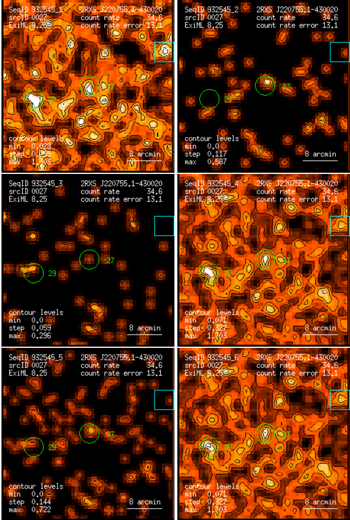
Figure 27: RASS 932545: detection 0027: band rate images, Gaussian filter: (1) PSPC channels 11 – 41, (2) 52 – 90, (3) 91 – 201, (4) 11 – 235, (5) 52 – 201, (6) 11 – 201. Broad band rates in counts/ks. Band rate contour levels in counts/ks/arcmin 2 .
