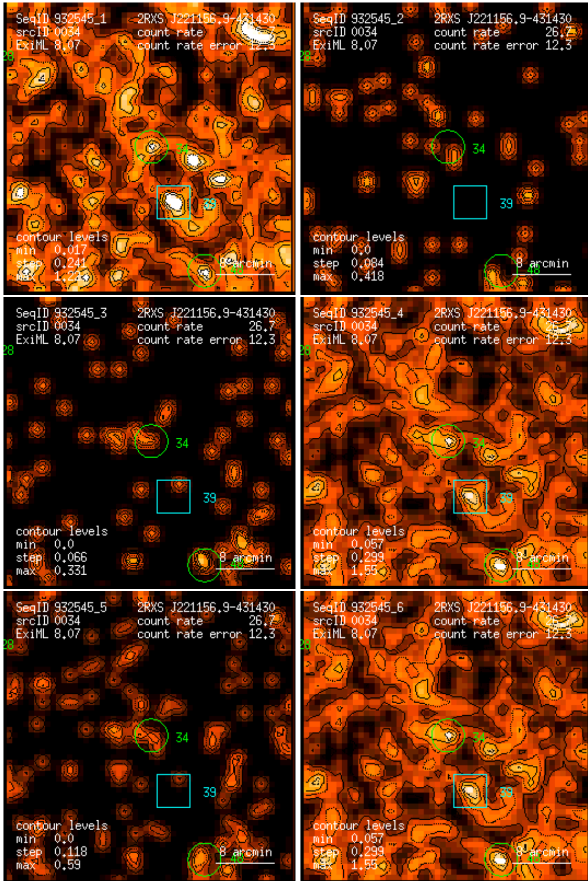
Figure 34: RASS 932545: detection 0034: band rate images, Gaussian filter: (1) PSPC channels 11 – 41, (2) 52 – 90, (3) 91 – 201, (4) 11 – 235, (5) 52 – 201, (6) 11 – 201. Broad band rates in counts/ks. Band rate contour levels in counts/ks/arcmin 2 .
