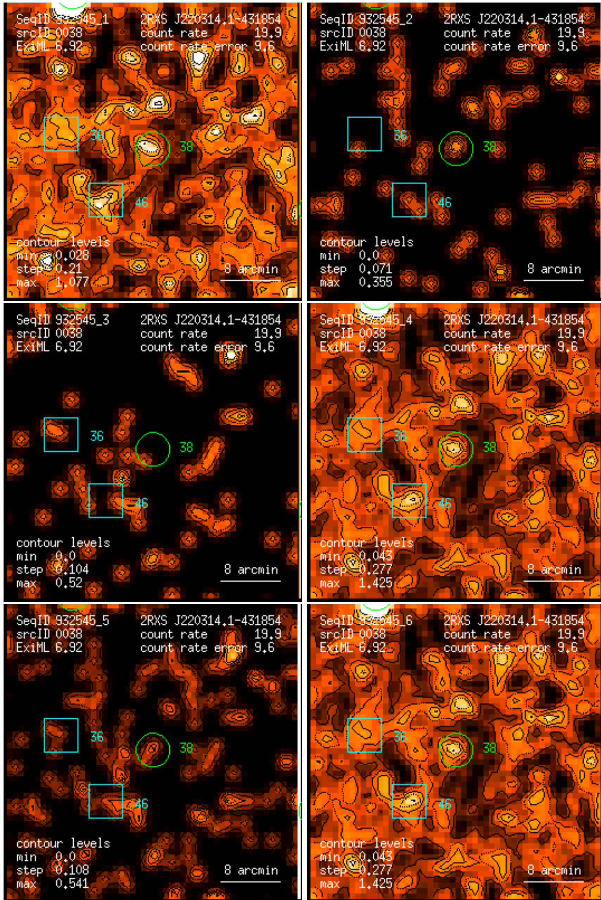
Figure 38: RASS 932545: detection 0038: band rate images, Gaussian filter: (1) PSPC channels 11 – 41, (2) 52 – 90, (3) 91 – 201, (4) 11 – 235, (5) 52 – 201, (6) 11 – 201. Broad band rates in counts/ks. Band rate contour levels in counts/ks/arcmin 2 .
