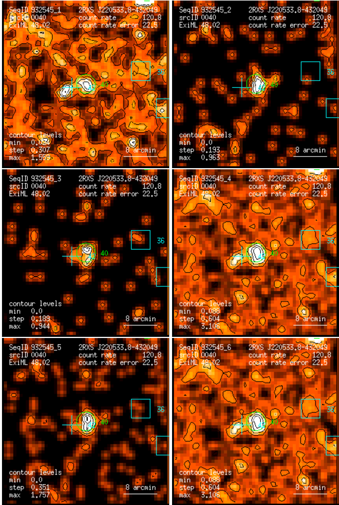
Figure 40: RASS 932545: detection 0040: band rate images, Gaussian filter: (1) PSPC channels 11 – 41, (2) 52 – 90, (3) 91 – 201, (4) 11 – 235, (5) 52 – 201, (6) 11 – 201. Broad band rates in counts/ks. Band rate contour levels in counts/ks/arcmin 2 .
