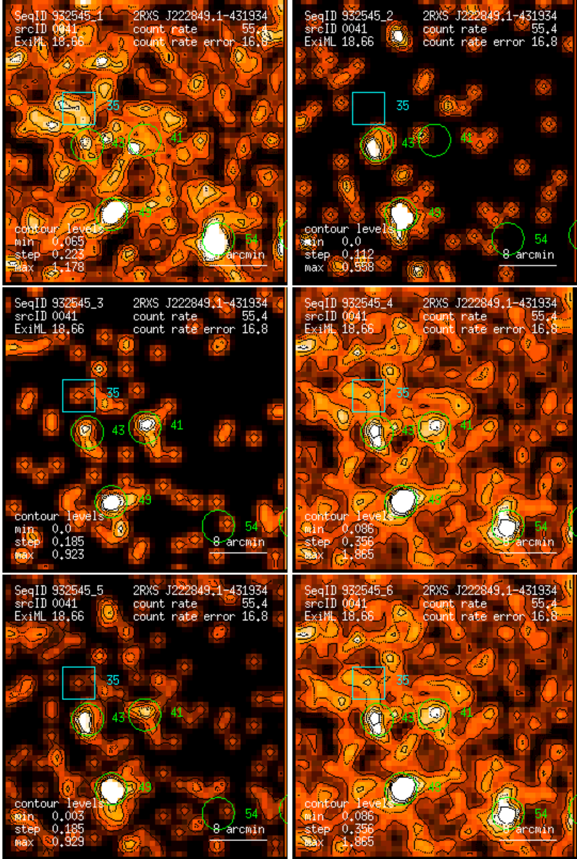
Figure 41: RASS 932545: detection 0041: band rate images, Gaussian filter: (1) PSPC channels 11 – 41, (2) 52 – 90, (3) 91 – 201, (4) 11 – 235, (5) 52 – 201, (6) 11 – 201. Broad band rates in counts/ks. Band rate contour levels in counts/ks/arcmin 2 .
