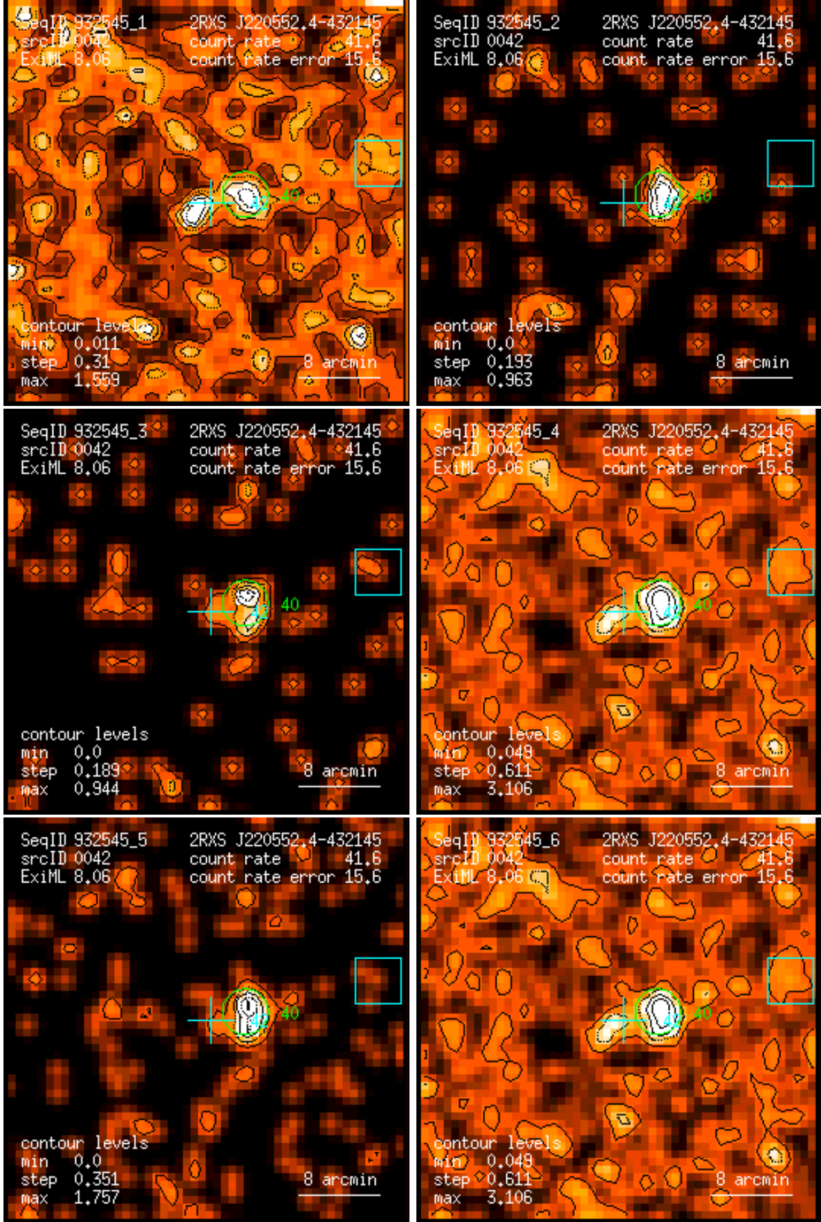
Figure 42: RASS 932545: detection 0042: band rate images, Gaussian filter: (1) PSPC channels 11 – 41, (2) 52 – 90, (3) 91 – 201, (4) 11 – 235, (5) 52 – 201, (6) 11 – 201. Broad band rates in counts/ks. Band rate contour levels in counts/ks/arcmin 2 .
