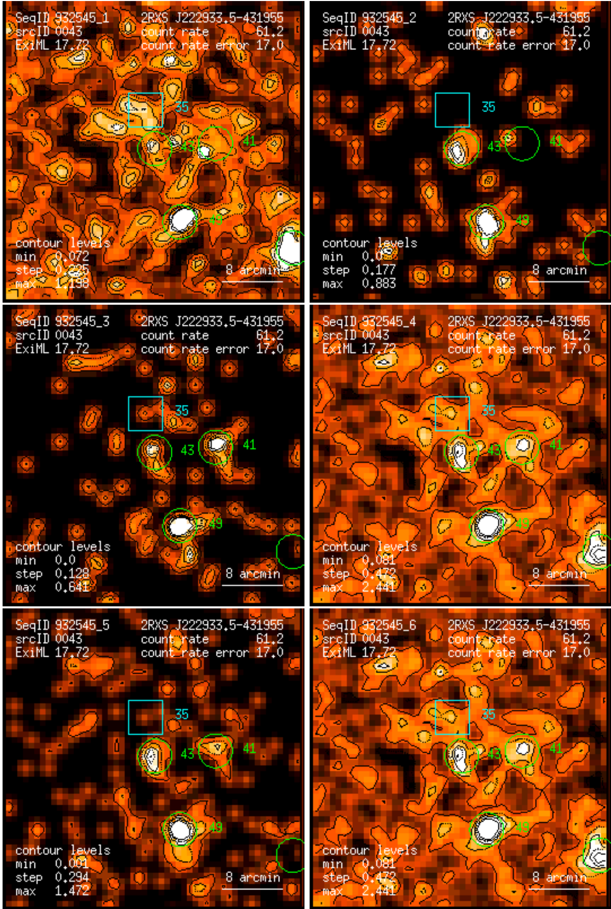
Figure 43: RASS 932545: detection 0043: band rate images, Gaussian filter: (1) PSPC channels 11 – 41, (2) 52 – 90, (3) 91 – 201, (4) 11 – 235, (5) 52 – 201, (6) 11 – 201. Broad band rates in counts/ks. Band rate contour levels in counts/ks/arcmin 2 .
