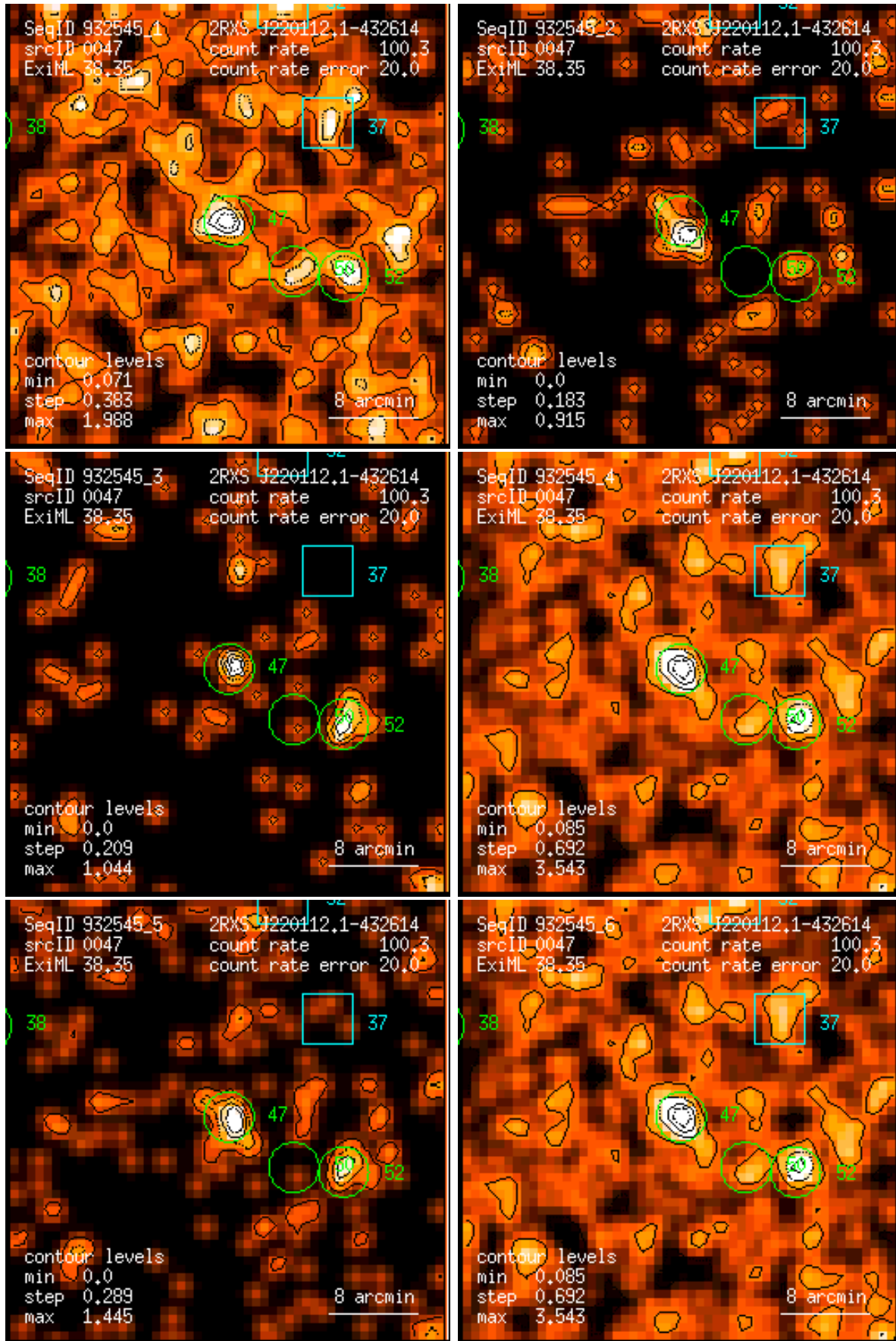
Figure 47: RASS 932545: detection 0047: band rate images, Gaussian filter: (1) PSPC channels 11 – 41, (2) 52 – 90, (3) 91 – 201, (4) 11 – 235, (5) 52 – 201, (6) 11 – 201. Broad band rates in counts/ks. Band rate contour levels in counts/ks/arcmin 2 .
