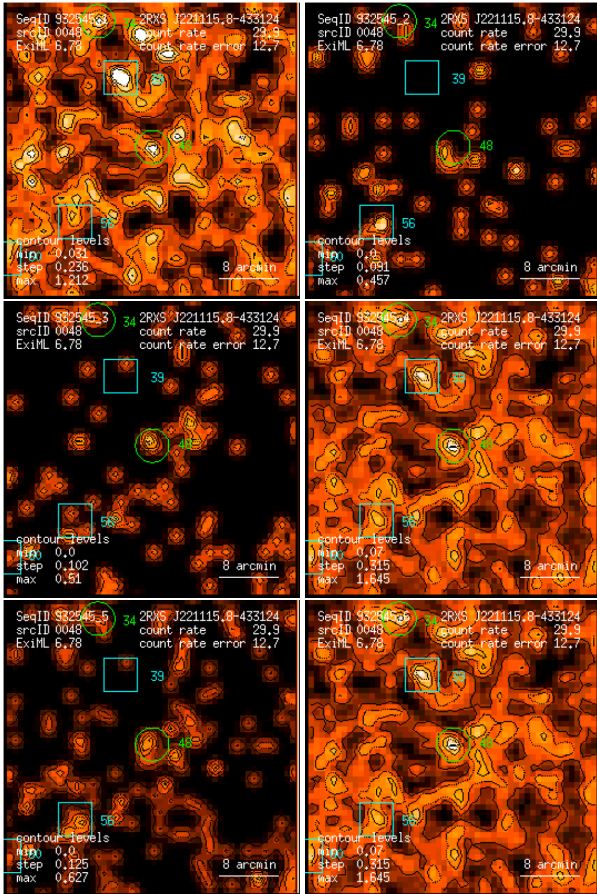
Figure 48: RASS 932545: detection 0048: band rate images, Gaussian filter: (1) PSPC channels 11 – 41, (2) 52 – 90, (3) 91 – 201, (4) 11 – 235, (5) 52 – 201, (6) 11 – 201. Broad band rates in counts/ks. Band rate contour levels in counts/ks/arcmin 2 .
