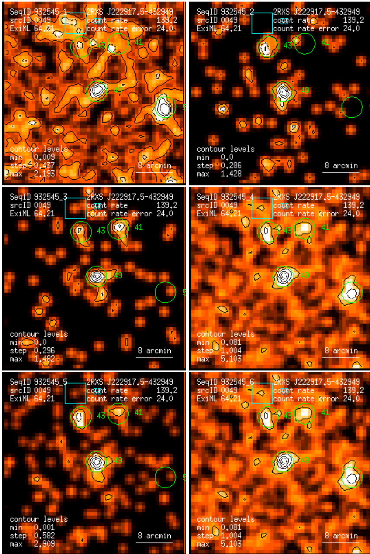
Figure 49: RASS 932545: detection 0049: band rate images, Gaussian filter: (1) PSPC channels 11 – 41, (2) 52 – 90, (3) 91 – 201, (4) 11 – 235, (5) 52 – 201, (6) 11 – 201. Broad band rates in counts/ks. Band rate contour levels in counts/ks/arcmin 2 .
