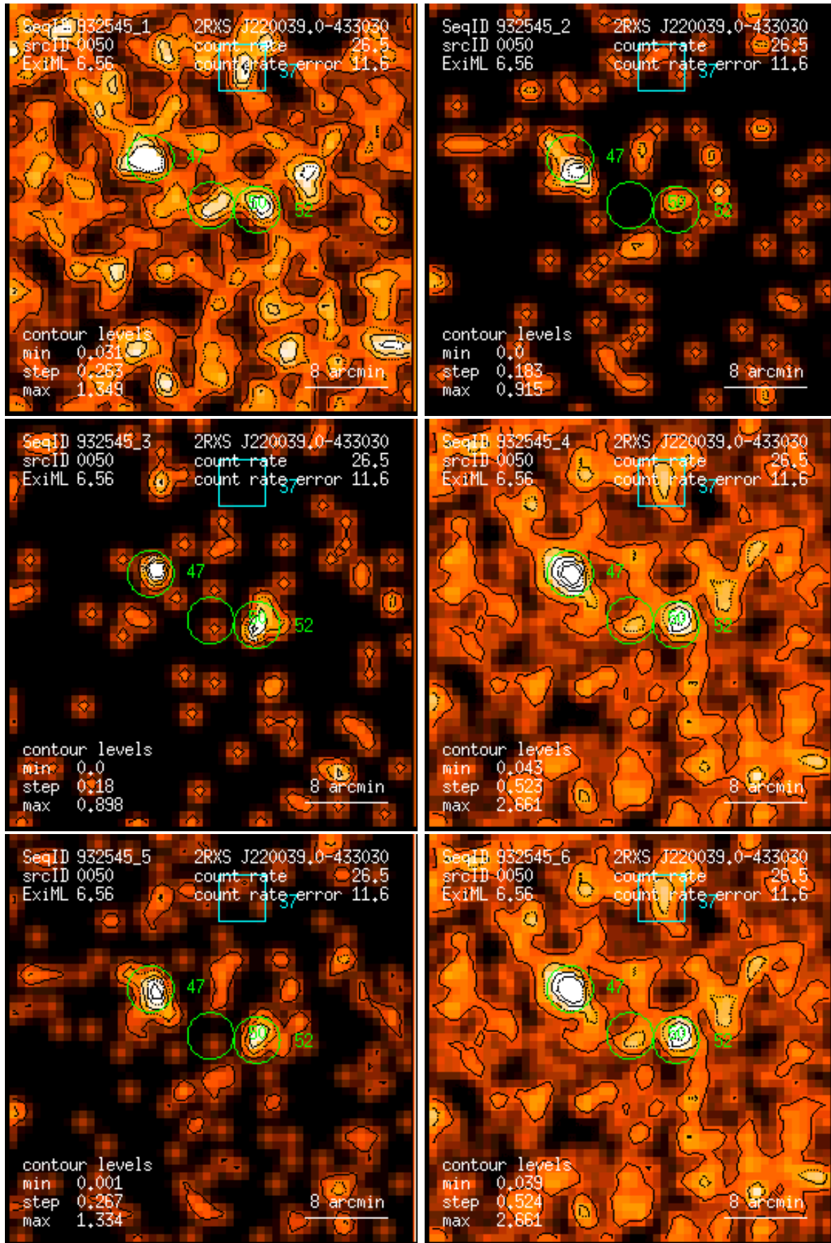
Figure 50: RASS 932545: detection 0050: band rate images, Gaussian filter: (1) PSPC channels 11 – 41, (2) 52 – 90, (3) 91 – 201, (4) 11 – 235, (5) 52 – 201, (6) 11 – 201. Broad band rates in counts/ks. Band rate contour levels in counts/ks/arcmin 2 .
