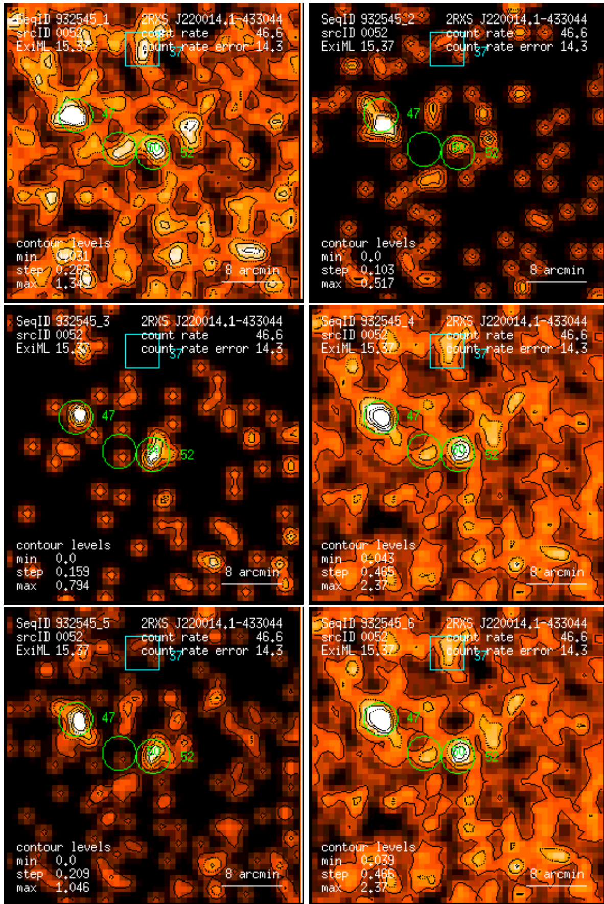
Figure 52: RASS 932545: detection 0052: band rate images, Gaussian filter: (1) PSPC channels 11 – 41, (2) 52 – 90, (3) 91 – 201, (4) 11 – 235, (5) 52 – 201, (6) 11 – 201. Broad band rates in counts/ks. Band rate contour levels in counts/ks/arcmin 2 .
