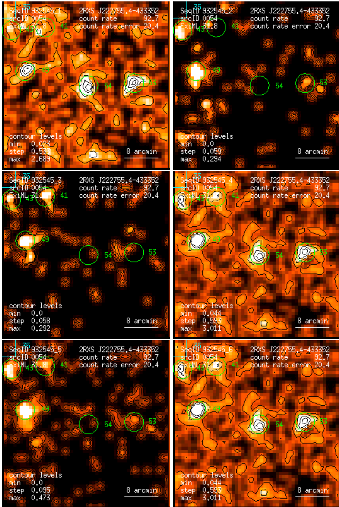
Figure 54: RASS 932545: detection 0054: band rate images, Gaussian filter: (1) PSPC channels 11 – 41, (2) 52 – 90, (3) 91 – 201, (4) 11 – 235, (5) 52 – 201, (6) 11 – 201. Broad band rates in counts/ks. Band rate contour levels in counts/ks/arcmin 2 .
