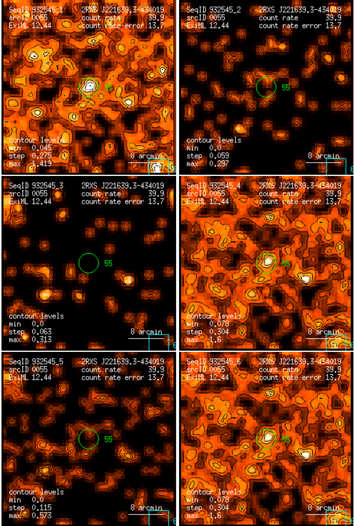
Figure 55: RASS 932545: detection 0055: band rate images, Gaussian filter: (1) PSPC channels 11 – 41, (2) 52 – 90, (3) 91 – 201, (4) 11 – 235, (5) 52 – 201, (6) 11 – 201. Broad band rates in counts/ks. Band rate contour levels in counts/ks/arcmin 2 .
