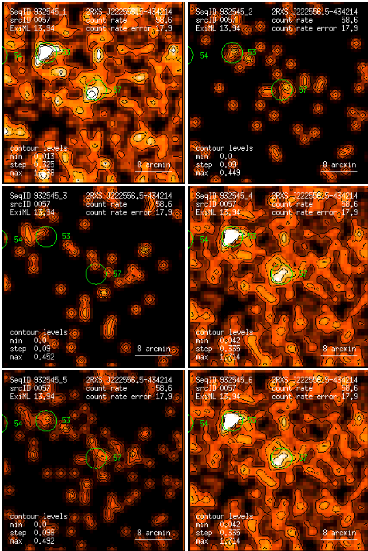
Figure 57: RASS 932545: detection 0057: band rate images, Gaussian filter: (1) PSPC channels 11 – 41, (2) 52 – 90, (3) 91 – 201, (4) 11 – 235, (5) 52 – 201, (6) 11 – 201. Broad band rates in counts/ks. Band rate contour levels in counts/ks/arcmin 2 .
