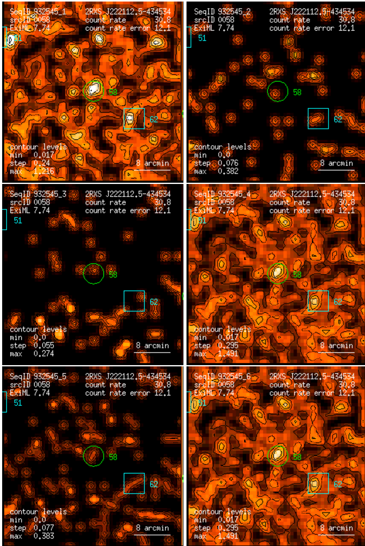
Figure 58: RASS 932545: detection 0058: band rate images, Gaussian filter: (1) PSPC channels 11 – 41, (2) 52 – 90, (3) 91 – 201, (4) 11 – 235, (5) 52 – 201, (6) 11 – 201. Broad band rates in counts/ks. Band rate contour levels in counts/ks/arcmin 2 .
