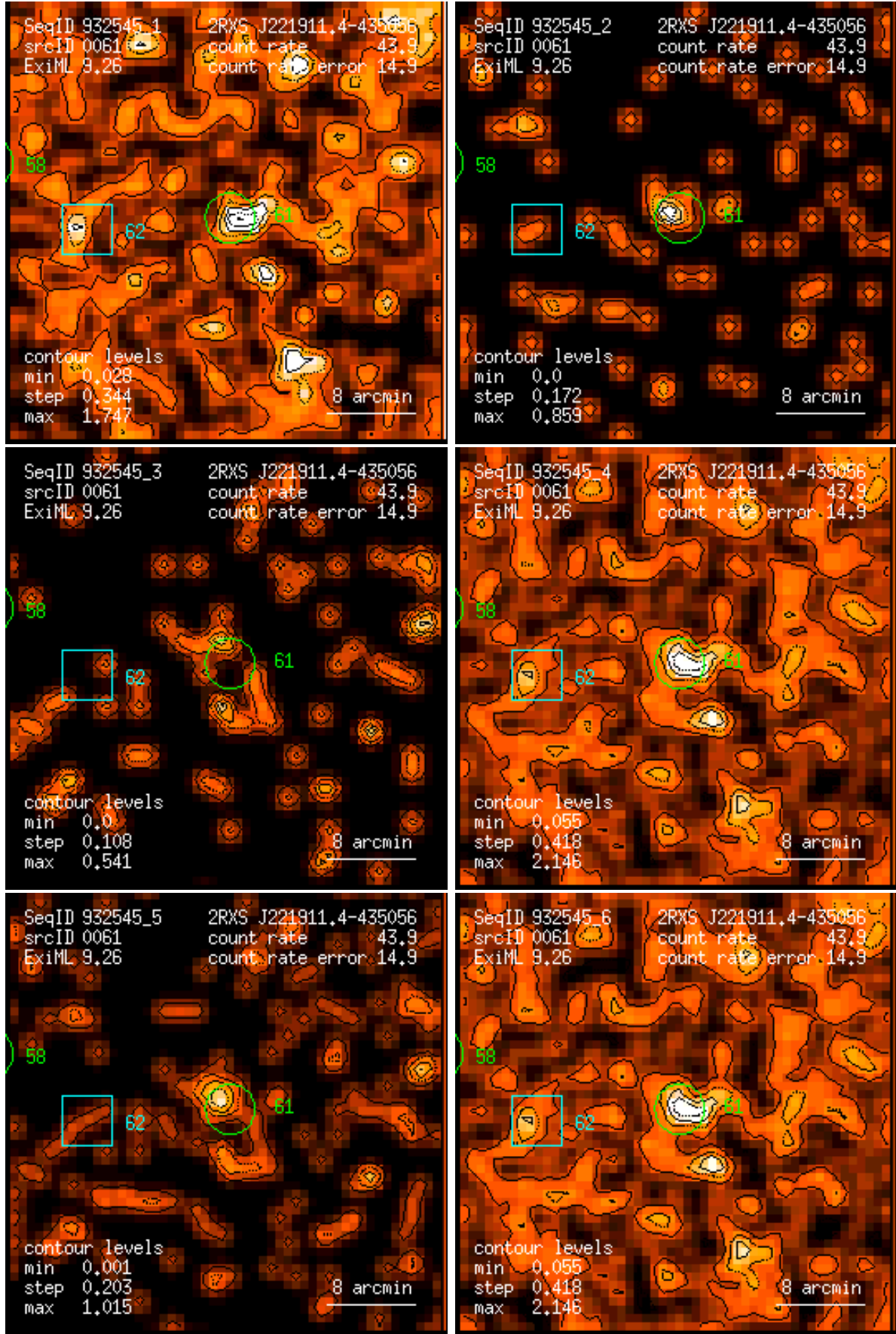
Figure 61: RASS 932545: detection 0061: band rate images, Gaussian filter: (1) PSPC channels 11 – 41, (2) 52 – 90, (3) 91 – 201, (4) 11 – 235, (5) 52 – 201, (6) 11 – 201. Broad band rates in counts/ks. Band rate contour levels in counts/ks/arcmin 2 .
