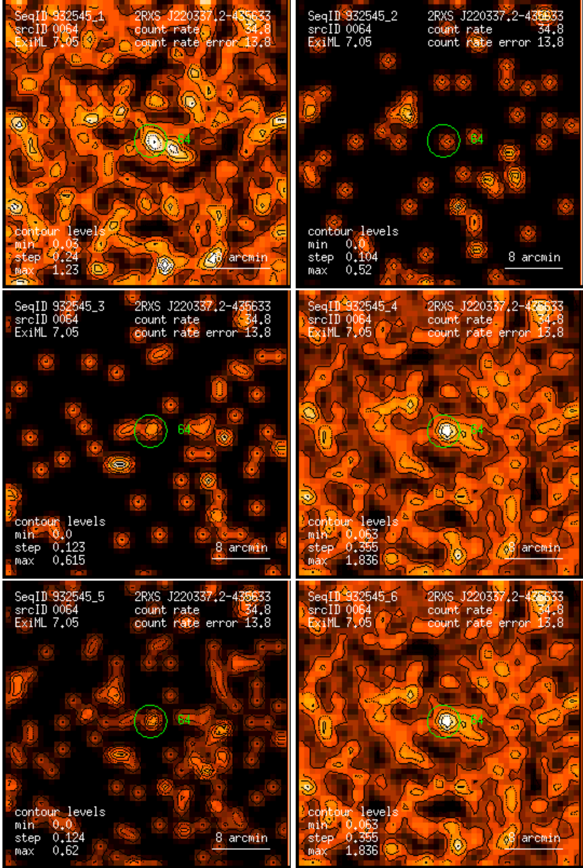
Figure 64: RASS 932545: detection 0064: band rate images, Gaussian filter: (1) PSPC channels 11 – 41, (2) 52 – 90, (3) 91 – 201, (4) 11 – 235, (5) 52 – 201, (6) 11 – 201. Broad band rates in counts/ks. Band rate contour levels in counts/ks/arcmin 2 .
