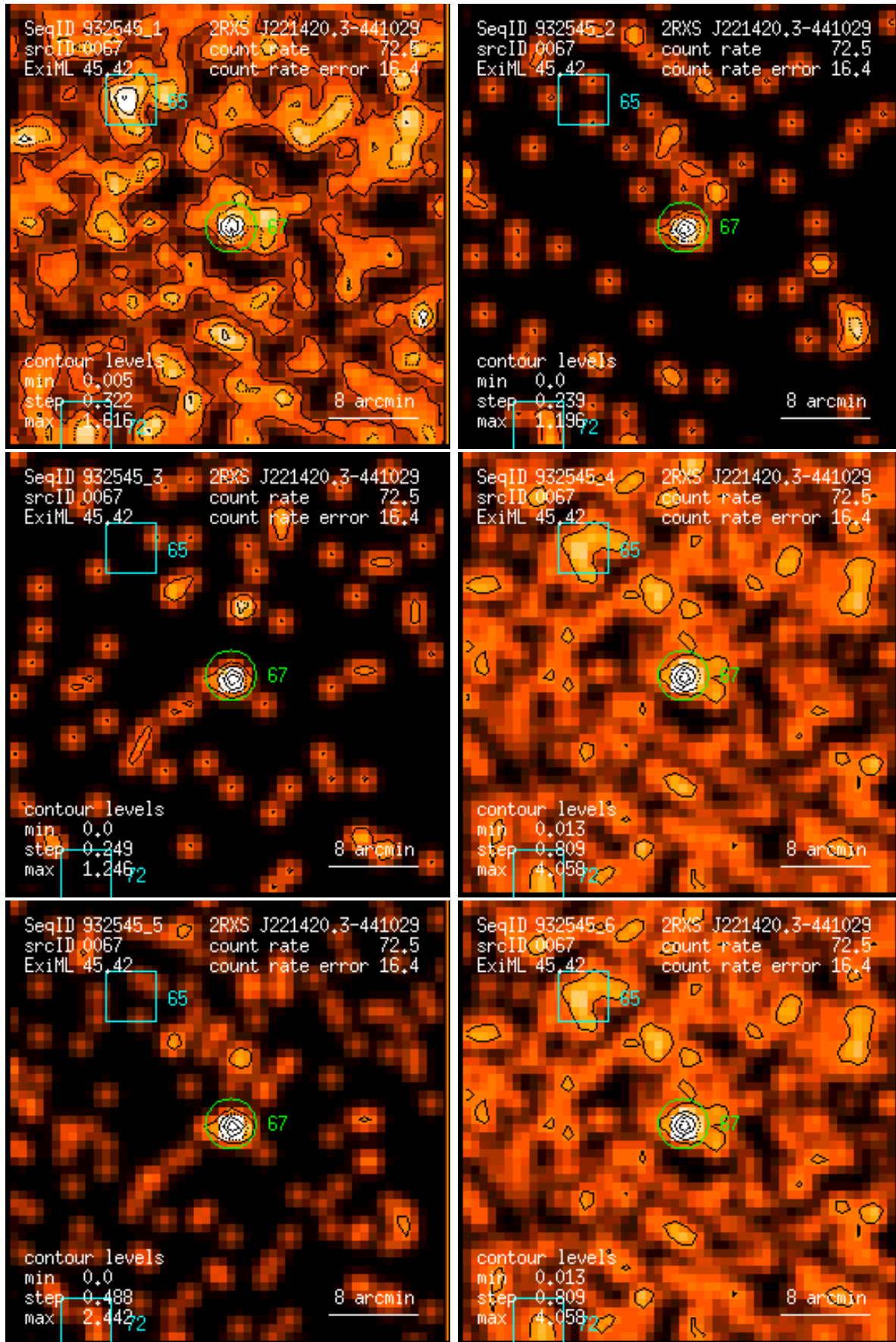
Figure 67: RASS 932545: detection 0067: band rate images, Gaussian filter: (1) PSPC channels 11 – 41, (2) 52 – 90, (3) 91 – 201, (4) 11 – 235, (5) 52 – 201, (6) 11 – 201. Broad band rates in counts/ks. Band rate contour levels in counts/ks/arcmin 2 .
