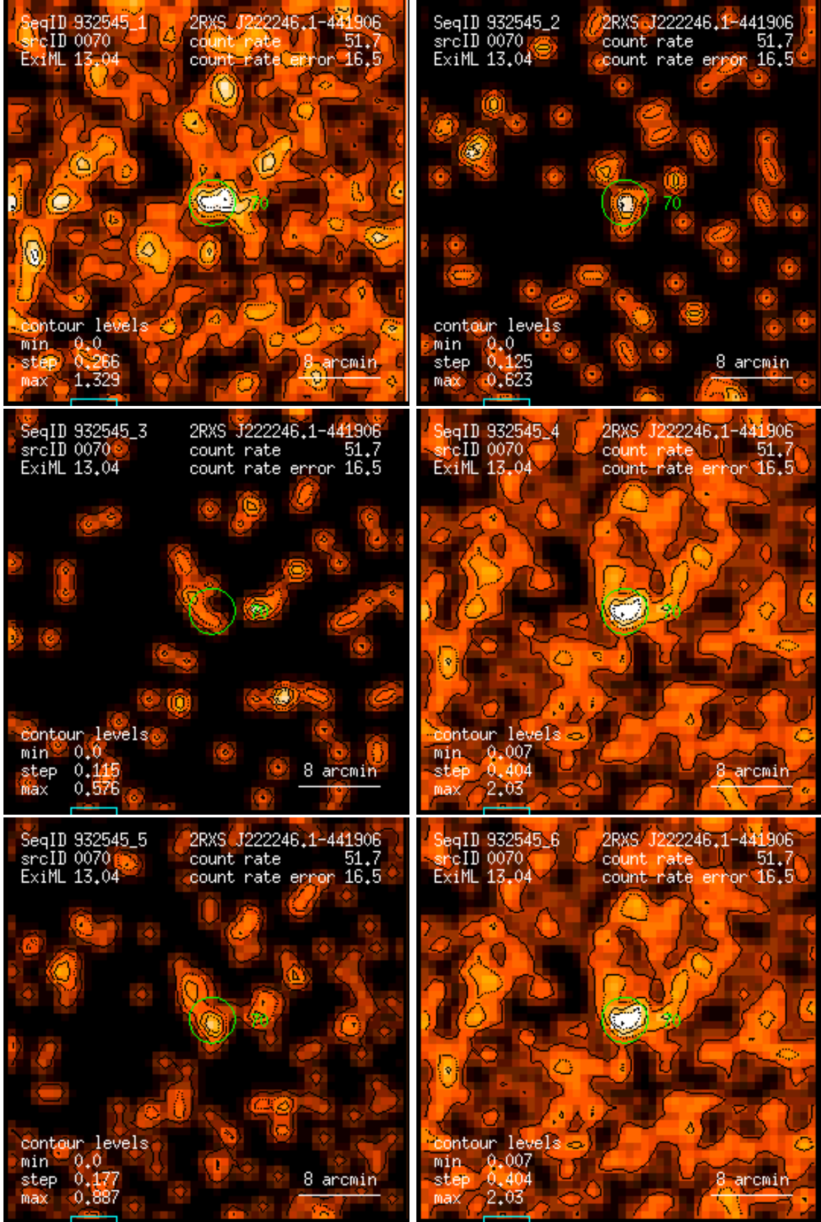
Figure 70: RASS 932545: detection 0070: band rate images, Gaussian filter: (1) PSPC channels 11 – 41, (2) 52 – 90, (3) 91 – 201, (4) 11 – 235, (5) 52 – 201, (6) 11 – 201. Broad band rates in counts/ks. Band rate contour levels in counts/ks/arcmin 2 .
